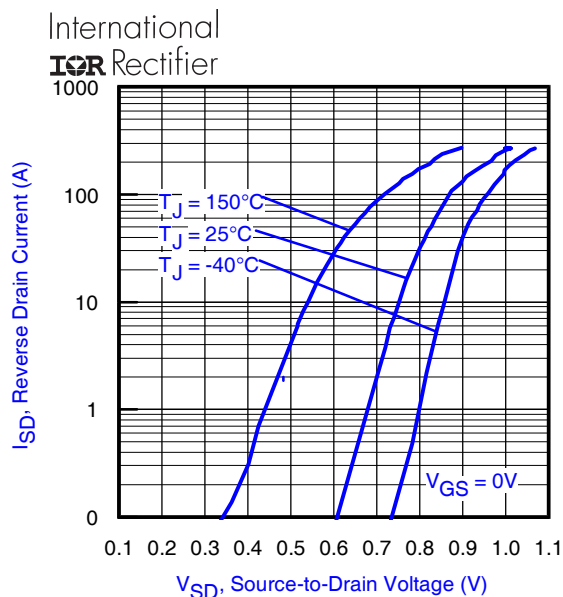
Fig 10. Typical Source-Drain Diode Forward Voltage
