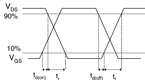
Fig 18b. Switching Time Waveforms
