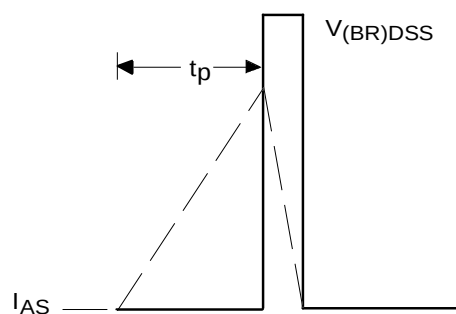
Fig 13c. Unclamped Inductive Waveforms
