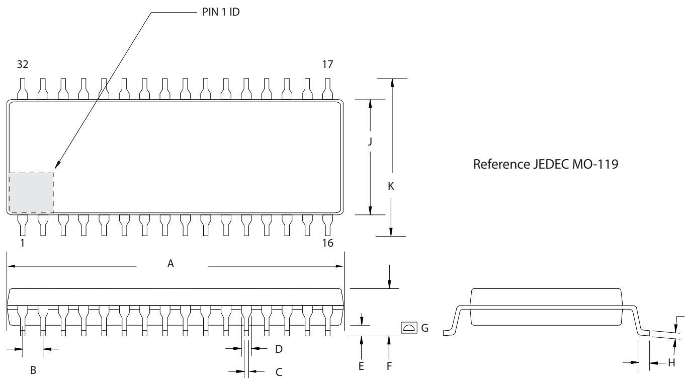
Figure 13 – 32-SOIC Package Outline 1
