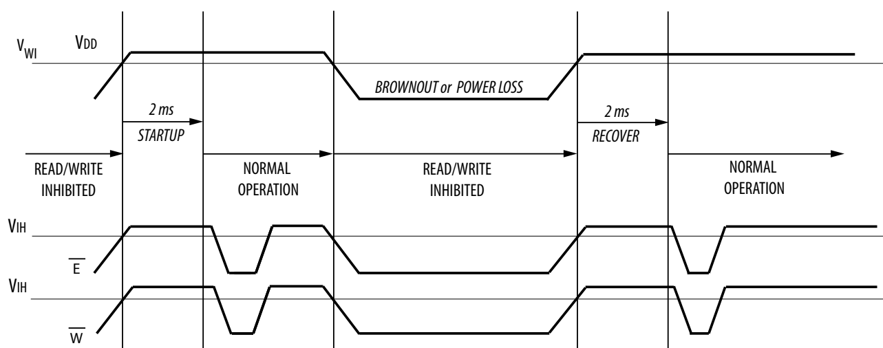
Figure 3 – Power Up and Power Down Diagram
