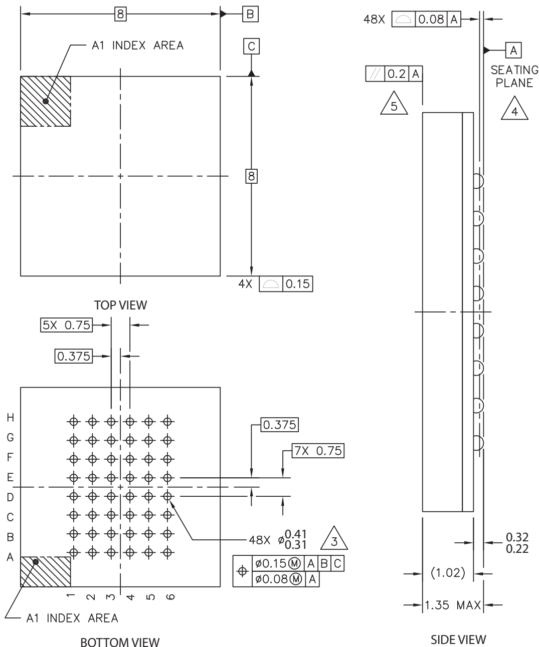
Figure 12 – 48-BGA Package Outline
