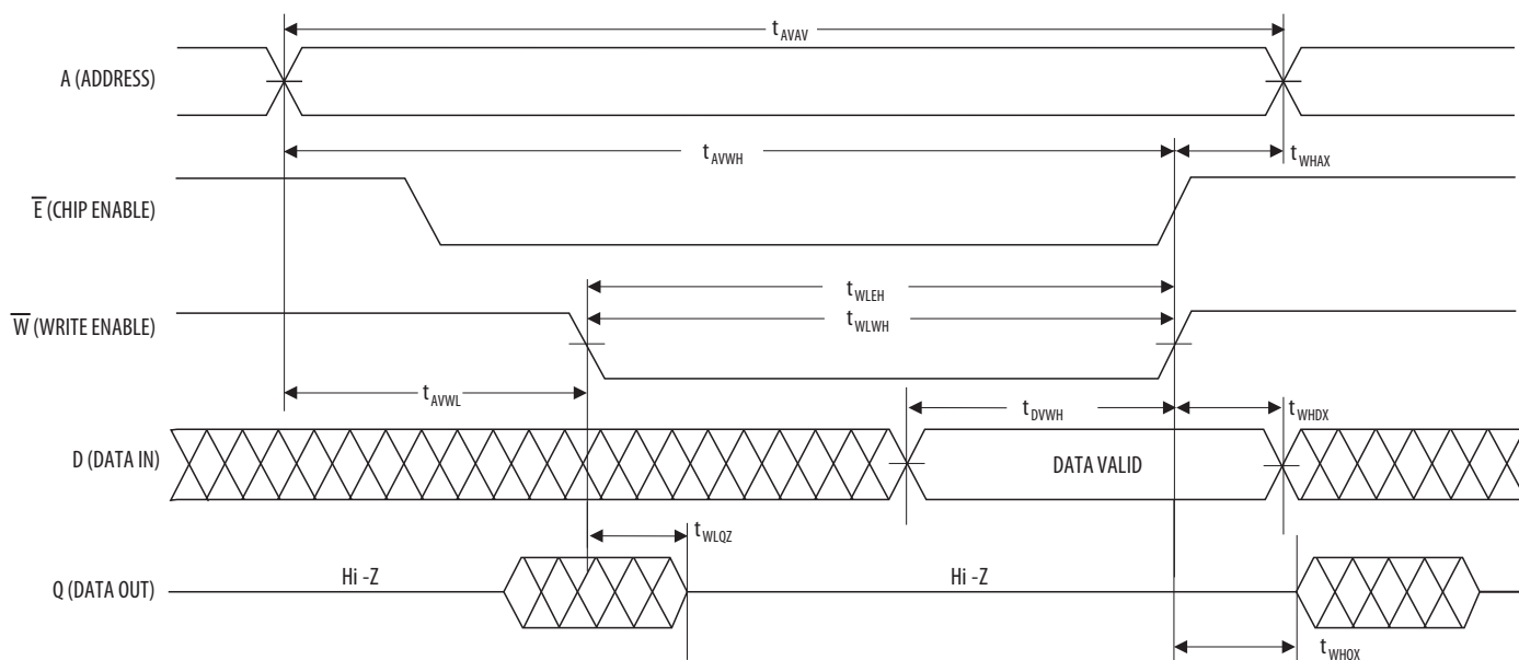
Figure 8 – Write Cycle Timing 1 ( \overline{W} Controlled)
