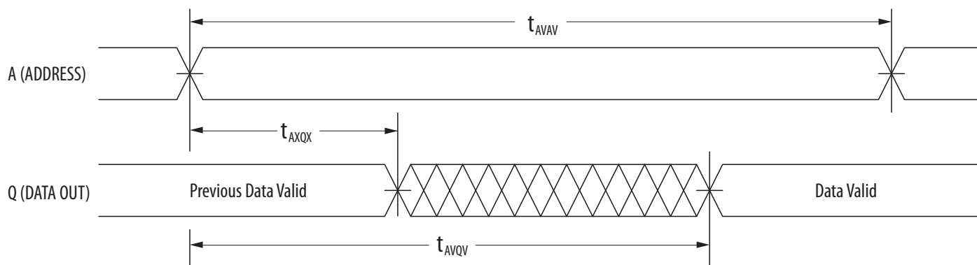
Figure 6 – Read Cycle 1
