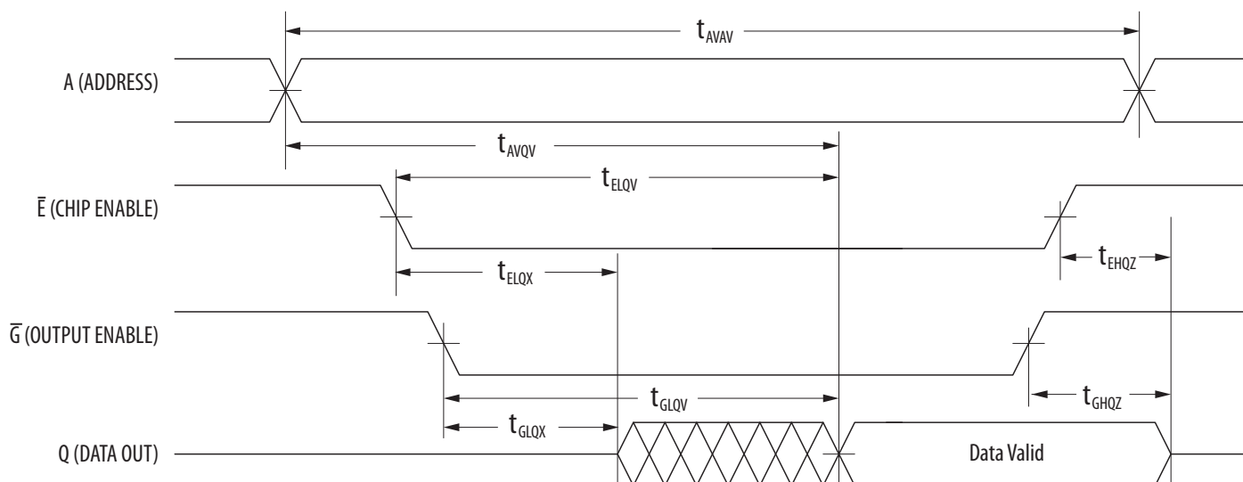
Figure 7 – Read Cycle 2
