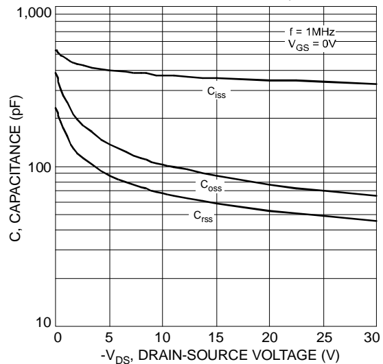
Fig. 15 Typical Capacitance
