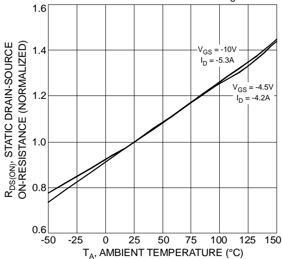
Fig. 14 On-Resistance Variation with Temperature
