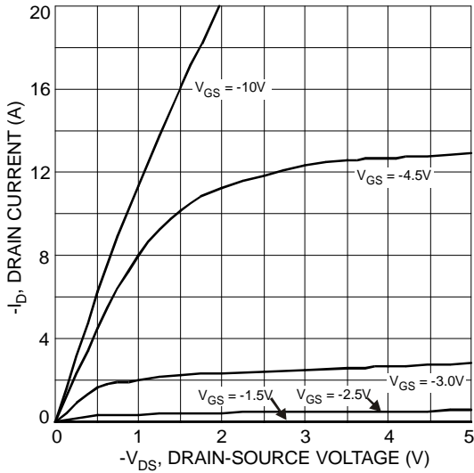
Fig. 10 Typical Output Characteristics
