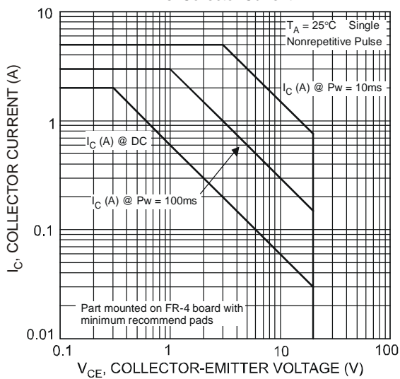
Fig. 7 Safe Operation Area
