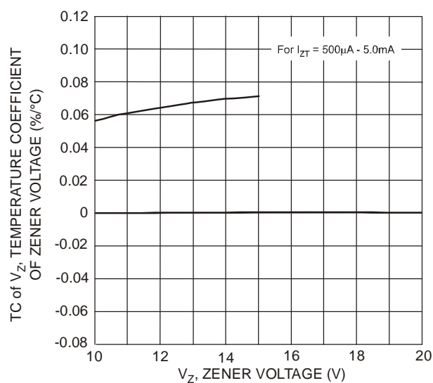
Fig. 8 Typical Temperature Coefficient of Zener Voltage vs. Zener Voltage, UDZ10B-UDZ15B
