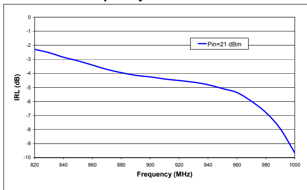
Figure 8. Input return loss vs frequency 13.6 V / 200 mA
