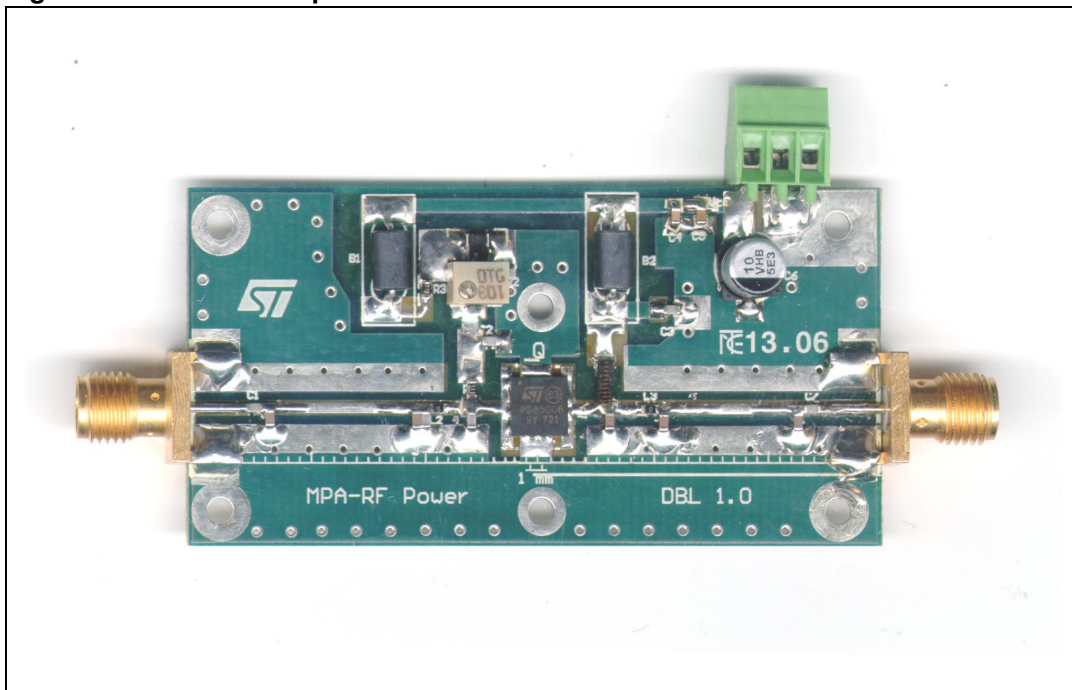
Figure 14. Demoboard photo
