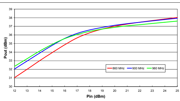
Figure 11. Pout vs pin 13.6 V / 200 mA
