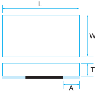
Short-side terminal
