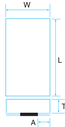
Long-side terminal
