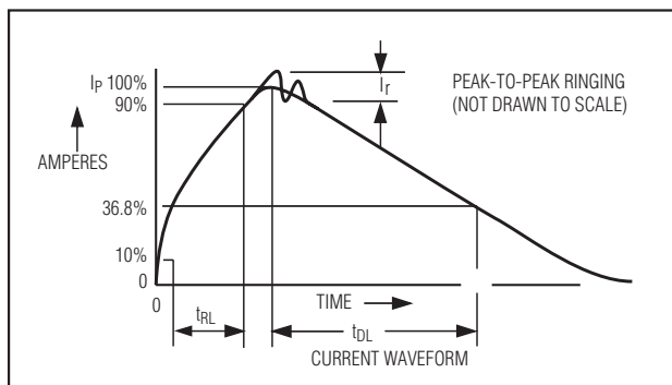
Figure 6. Human Body Current Waveform
