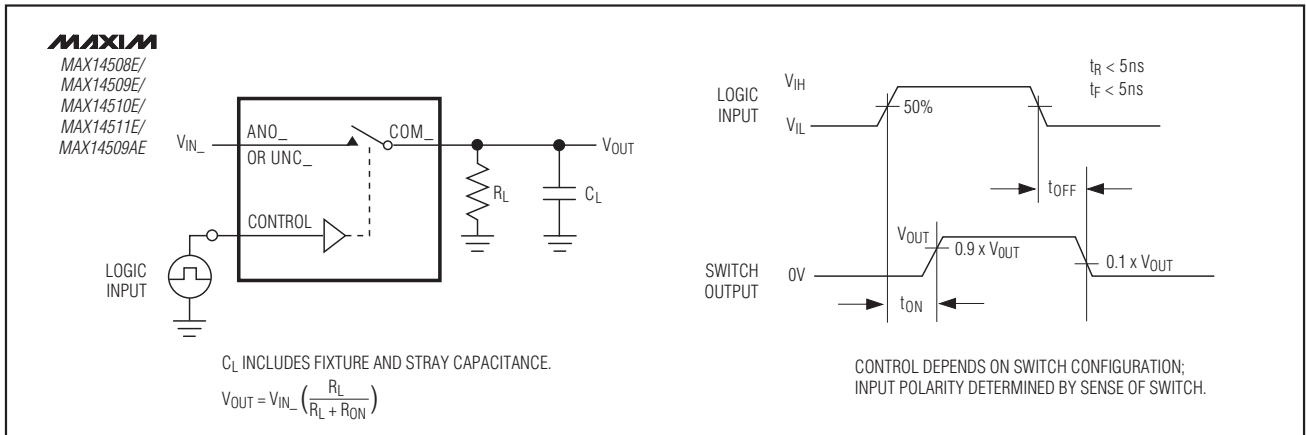
Figure 2. Switching Time
