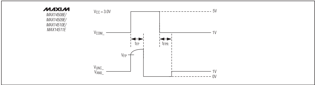
Figure 1. Fault Protection
