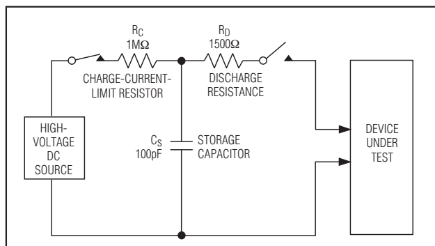
Figure 5. Human Body ESD Test Model
