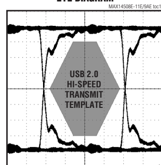
EYE DIAGRAM
