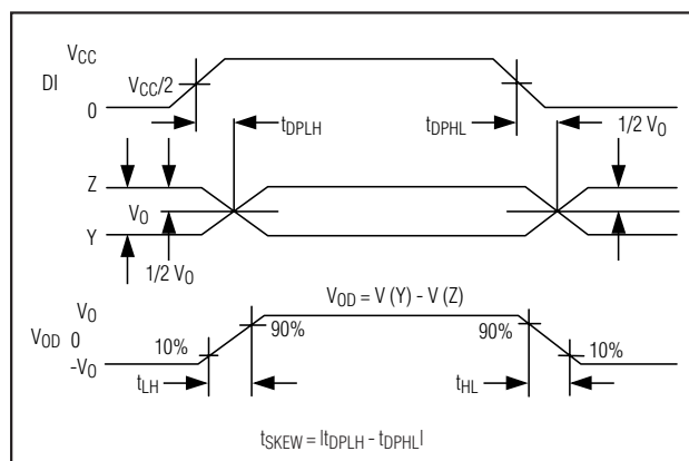
Figure 3. Driver Propagation Delays
