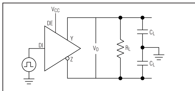
Figure 2. Driver Timing Test Circuit
