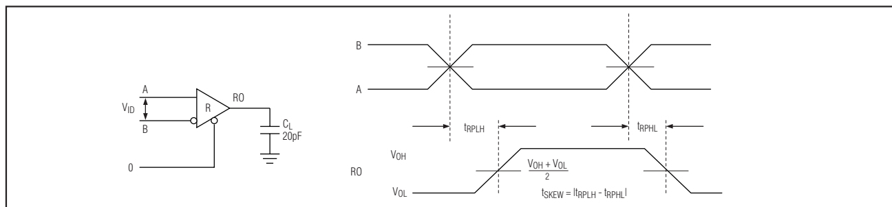
Figure 6. Receiver Propagation Delays
