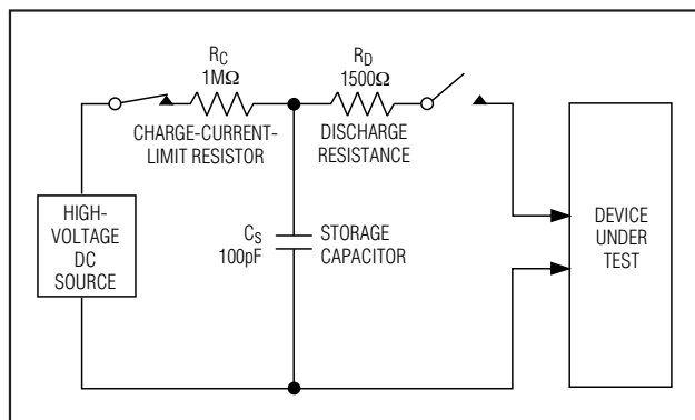
Figure 8a. Human Body ESD Test Model
