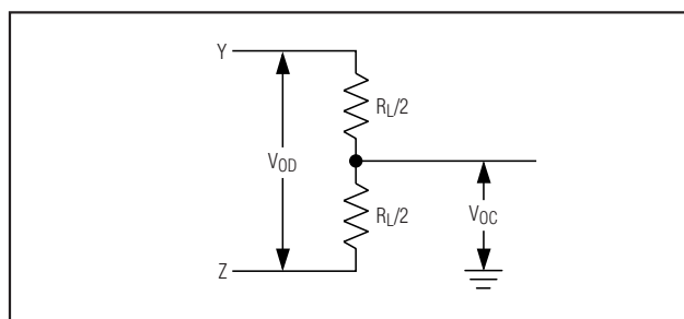
Figure 1. Driver DC Test Load
