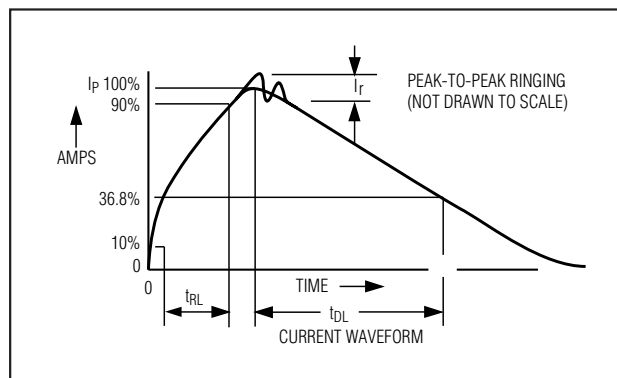
Figure 8b. Human Body Current Waveform
