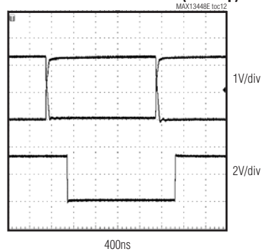
RECEIVER PROPAGATION DELAY (500kbsp)
