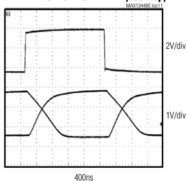
DRIVER PROPAGATION DELAY (500kbsp)
