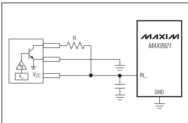
Figure 6. 3-Wire Hall-Effect Switches Configured as 2-Wire
