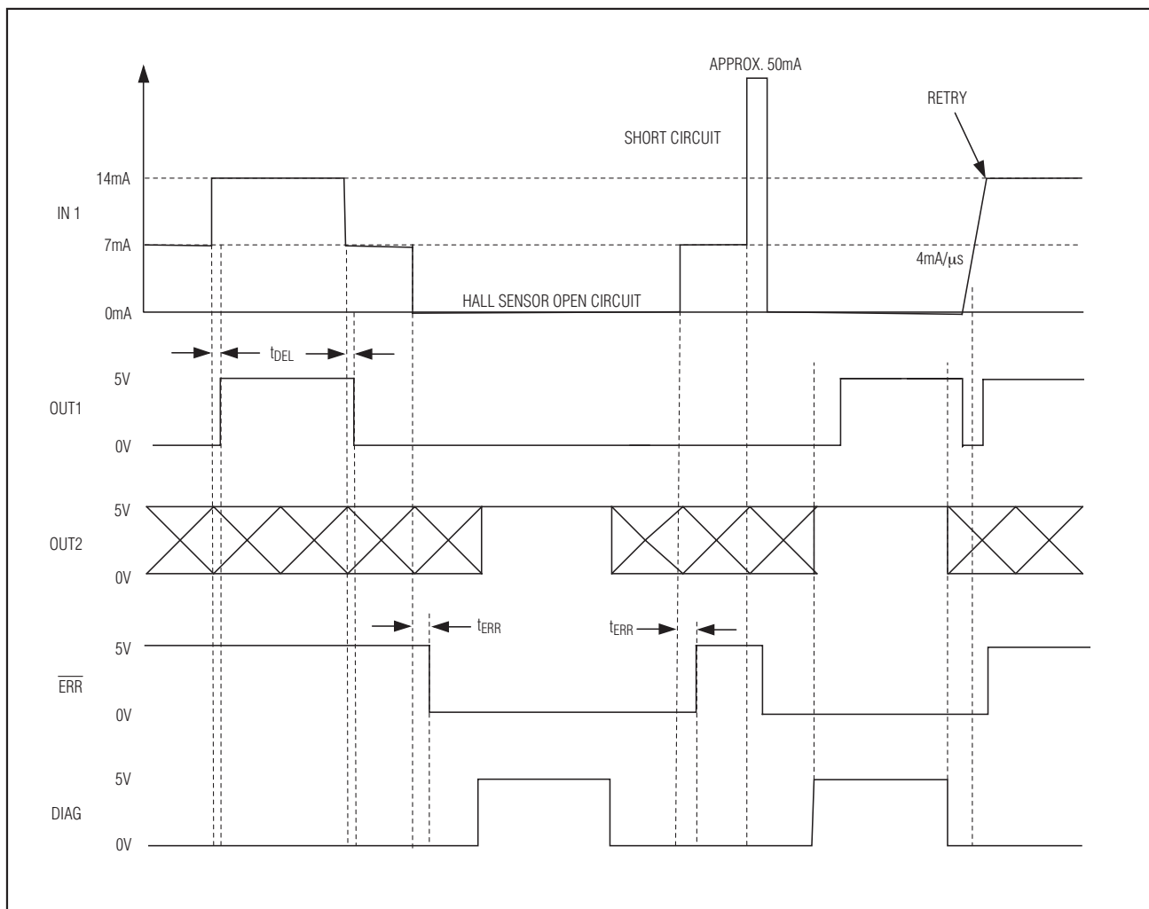
Figure 1. Timing Diagram
