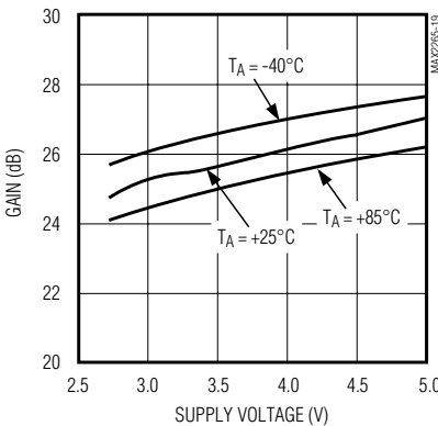
MAX2265 GAIN vs. SUPPLY VOLTAGE
