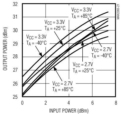
MAX2265 OUTPUT POWER vs. INPUT POWER
