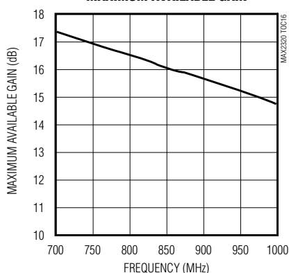
CELLULAR-BAND HGHL LNA MAXIMUM AVAILABLE GAIN
