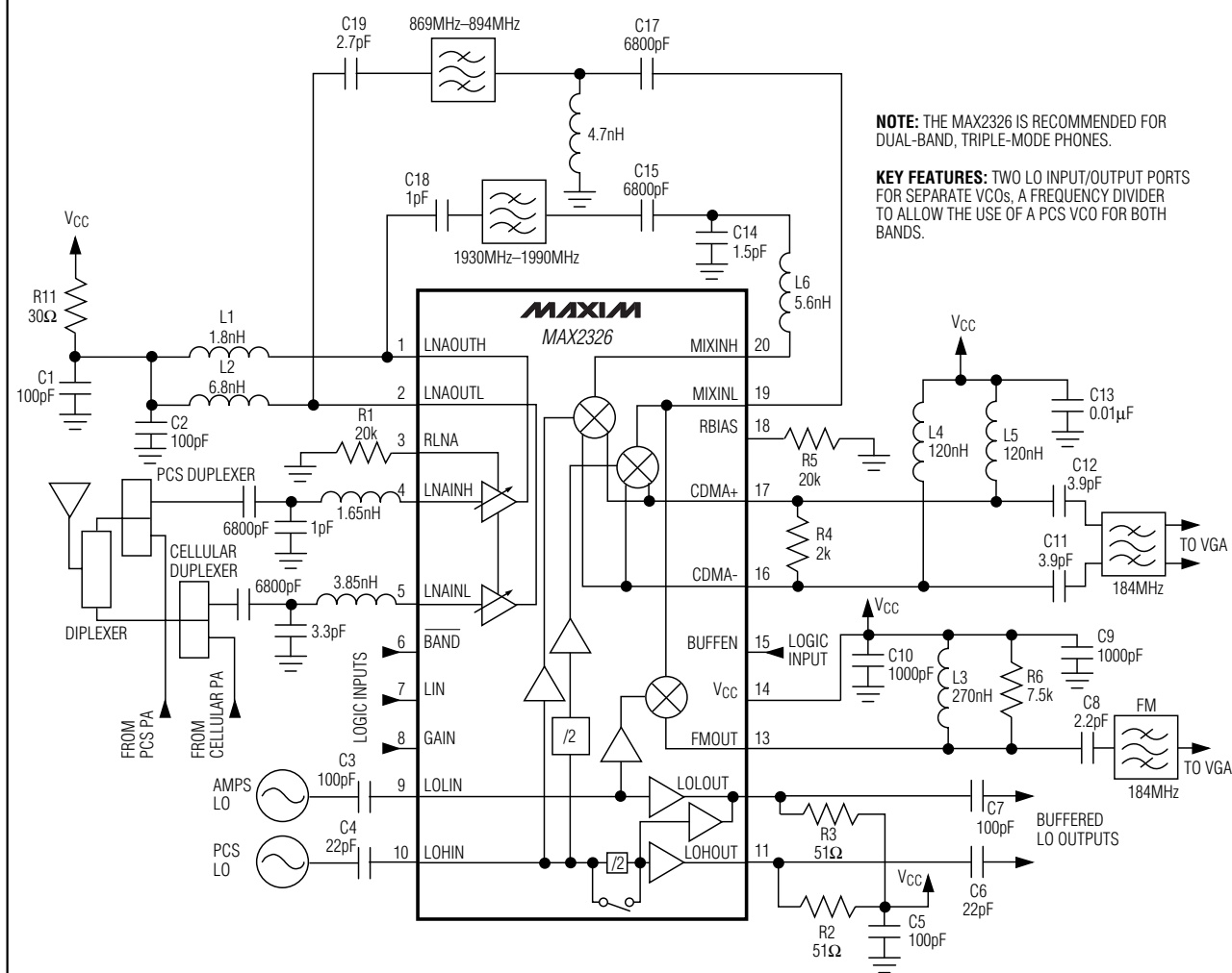
MAX2326 (DUAL BAND, DUAL VCO INPUTS, AND DUAL IF OUTPUTS WITH LO DIVIDER)
