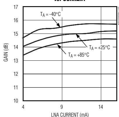
PCS-BAND HGHL LNA GAIN vs. CURRENT
