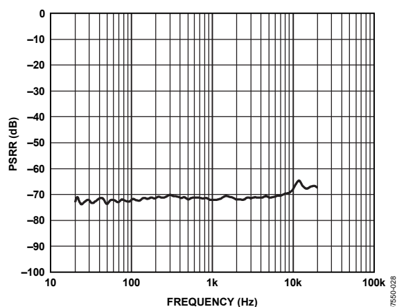
Figure 28. Power Supply Rejection Ratio (PSRR) vs. Frequency
