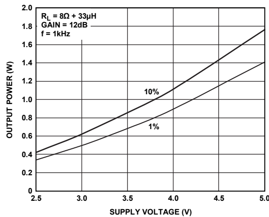
Figure 18. Maximum Output Power vs. Supply Voltage, R_L = 8\Omega + 33\mu H , Gain = 12 dB
