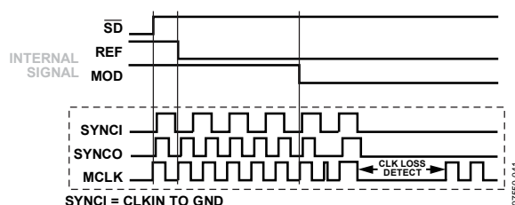
Figure 41. SYNCI = Clock Input to GND
