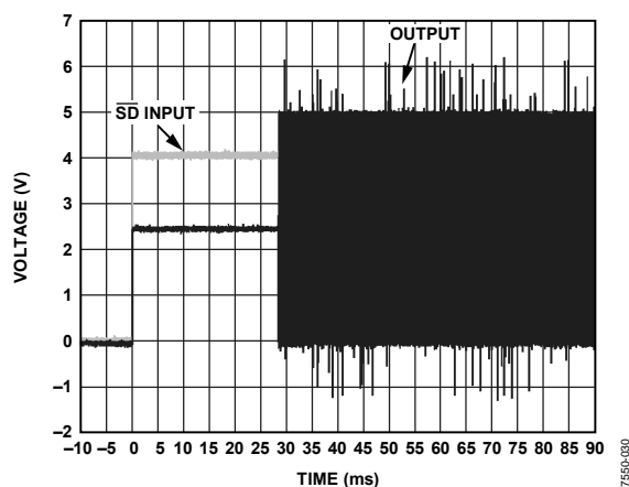
Figure 30. Turn-On Response
