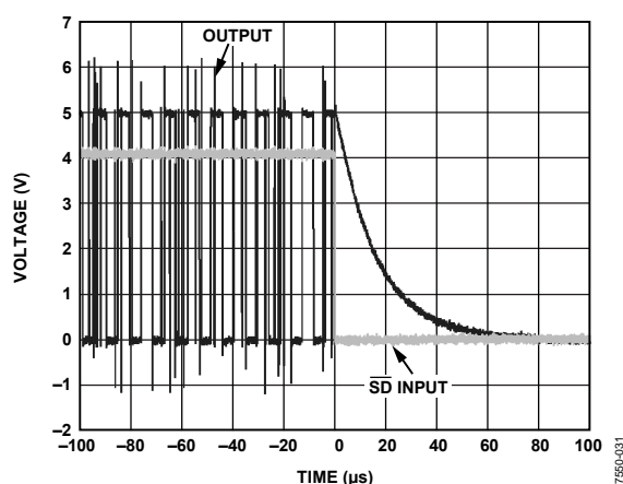
Figure 31. Turn-Off Response
