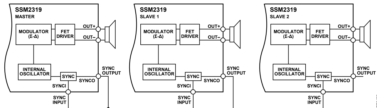
Figure 35. Typical SYNC Master-Slave Daisy-Chain Configuration
