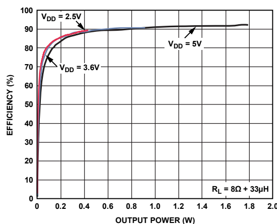
Figure 19. Efficiency vs. Output Power into R_L = 8\Omega + 33\mu H
