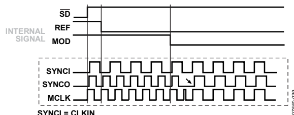
Figure 39. SYNCI = External Clock
