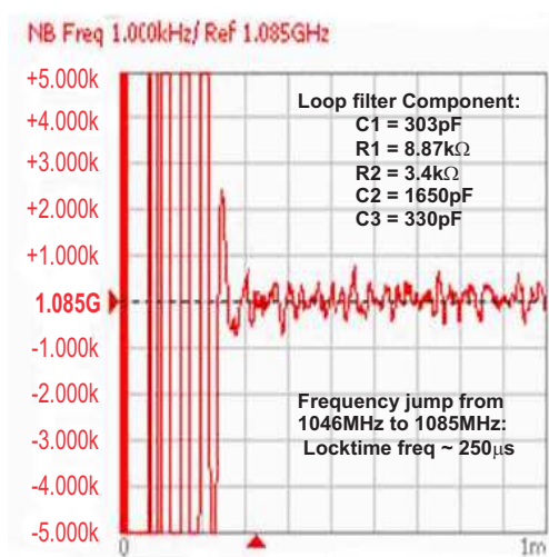
Figure 88. Frequency Locktime
