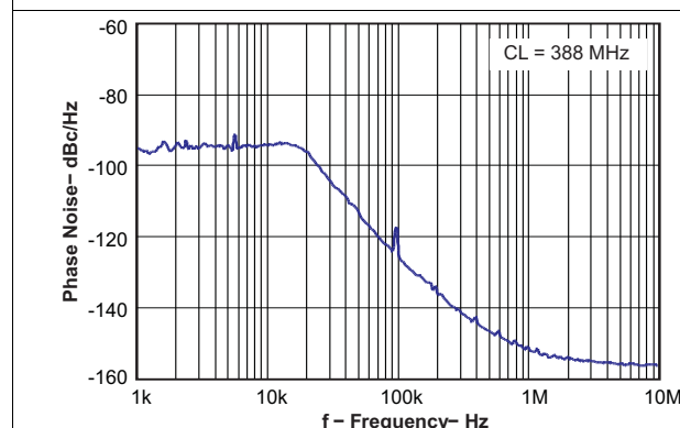
Figure 6. Closed Loop VCO Phase Noise
