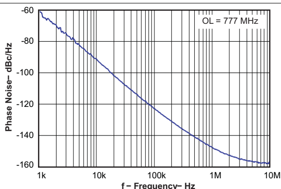
Figure 5. Open Loop VCO Phase Noise
