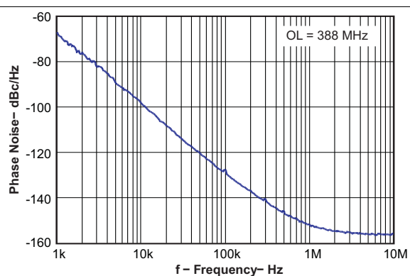
Figure 7. Open Loop VCO Phase Noise
