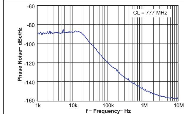
Figure 4. Closed Loop VCO Phase Noise
