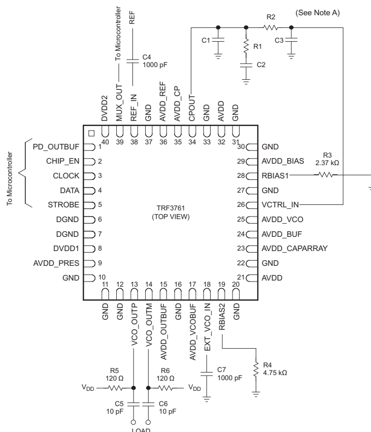
Figure 87. TRF3761 Application Schematic
