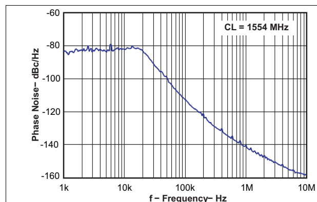
Figure 2. Closed Loop VCO Phase Noise
