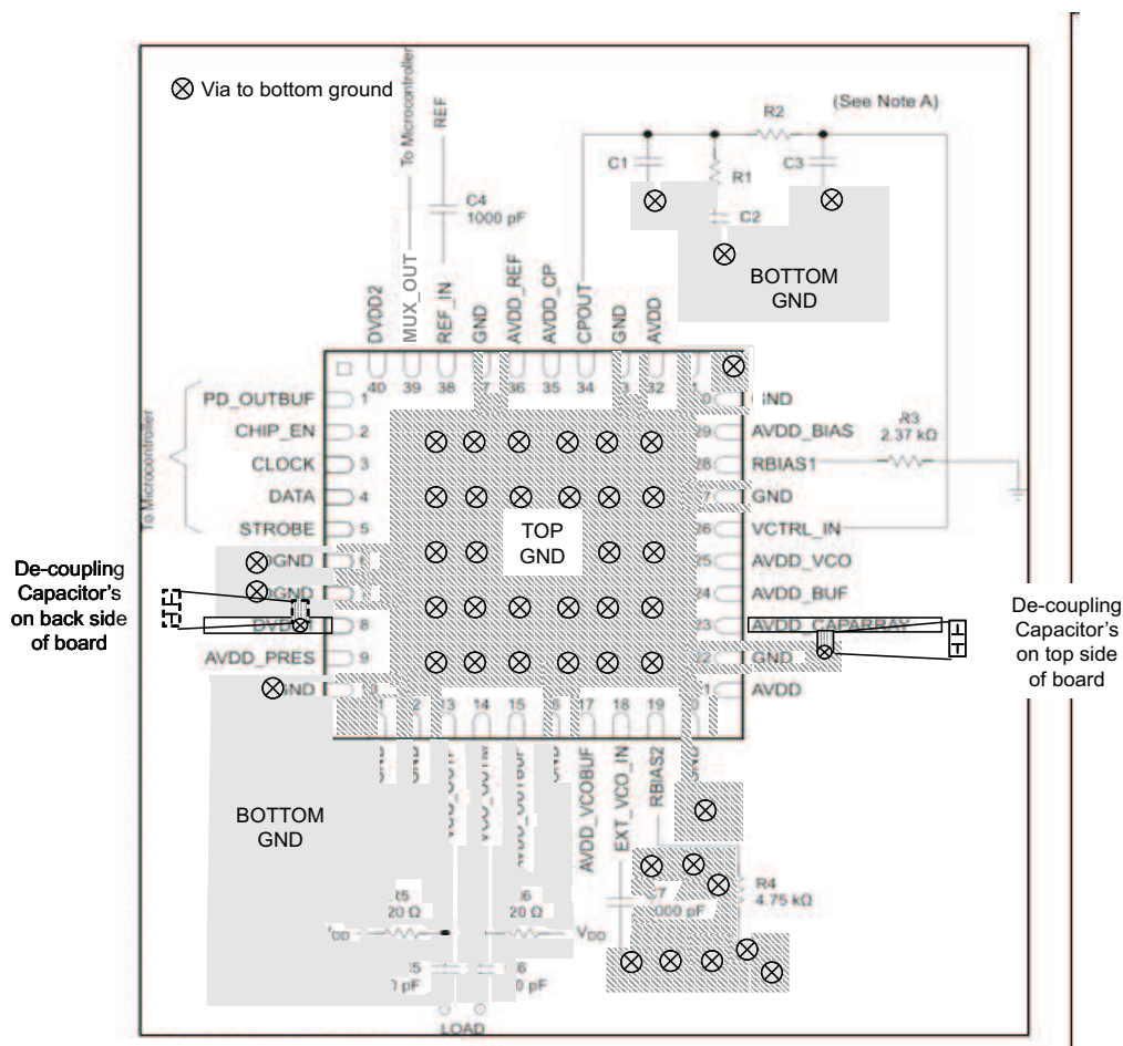
Figure 91. TRF3761 Layout
