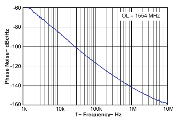
Figure 3. Open Loop VCO Phase Noise
