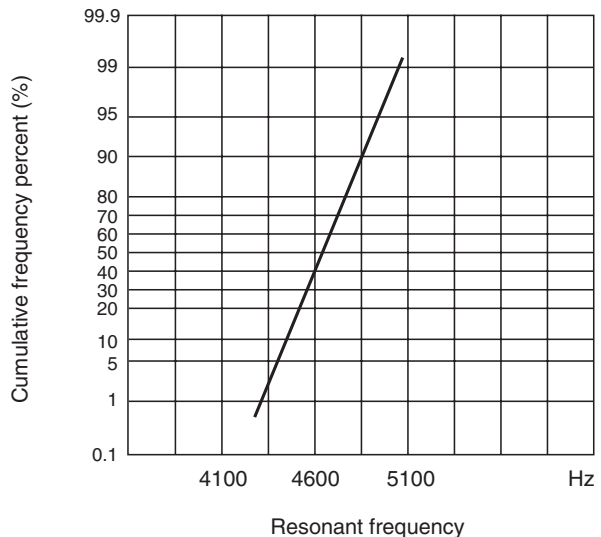
(4) Resonant frequency
