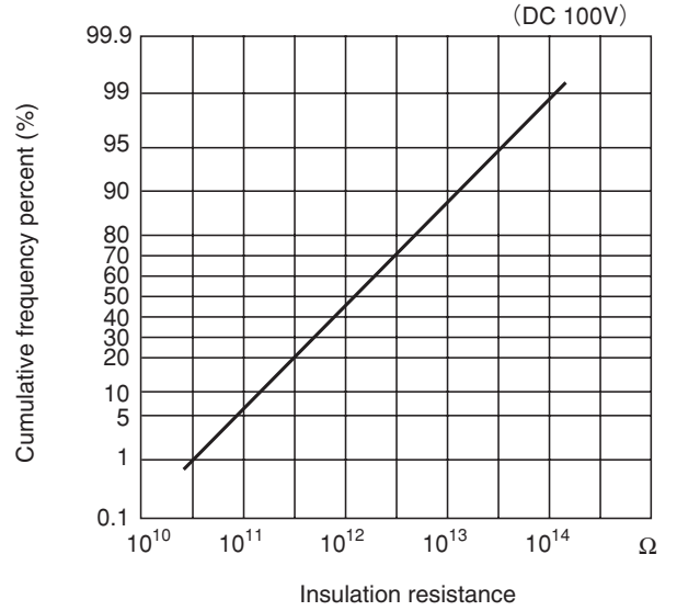
(4) Insulation resistance
