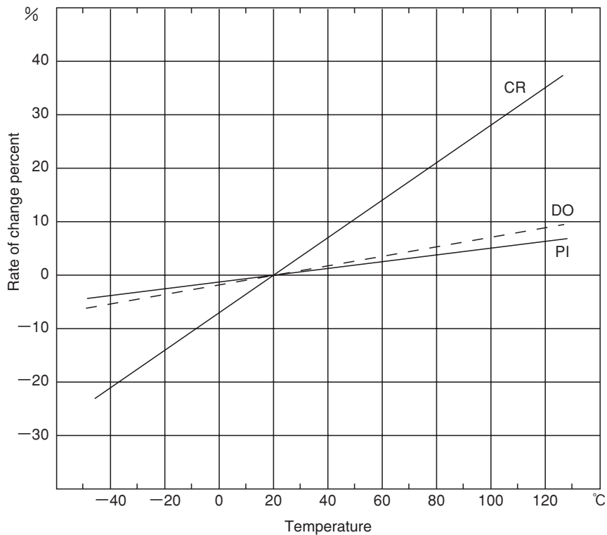
(1) Temperature characteristics
