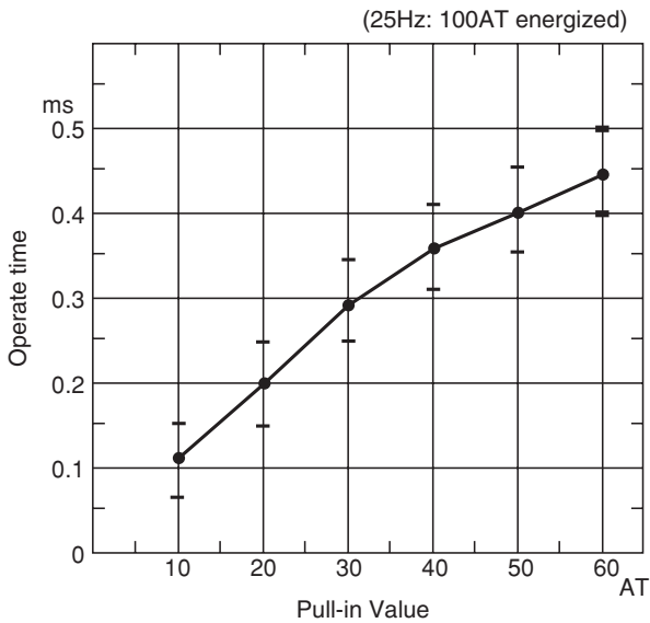
(1) Operate time
