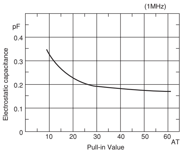
(5) Electrostatic capacitance
