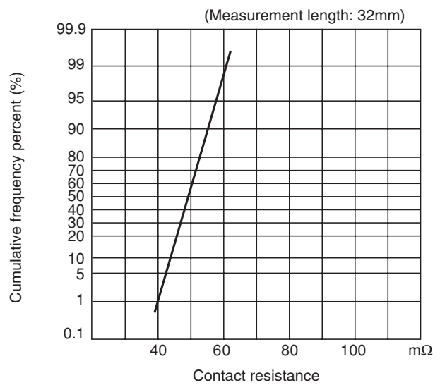
(2) Contact resistance
