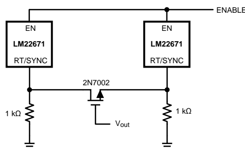
Figure 14. Self-Synchronizing Setup
