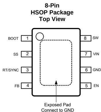
Pin Functions
