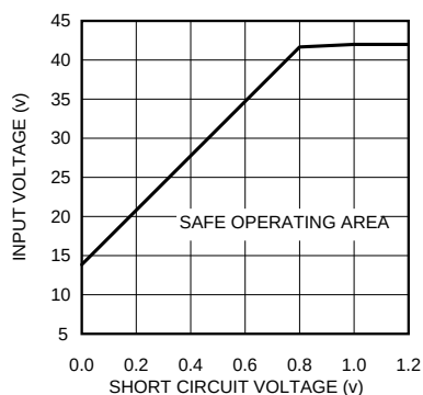
Figure 18. SOA at 800 kHz
