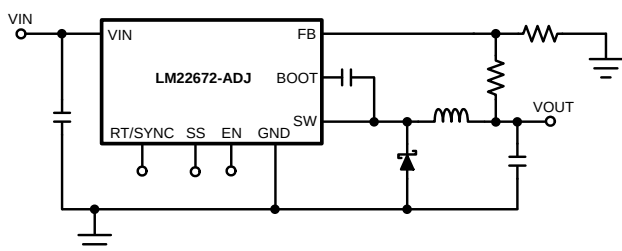
Simplified Application Schematic
