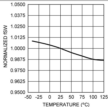
Figure 2. Normalized Switching Frequency vs Temperature
