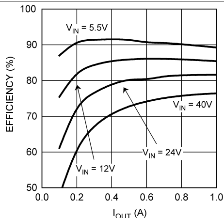
Figure 1. Efficiency vs I_{OUT} and V_{IN} , V_{OUT} = 3.3\text{ V}
