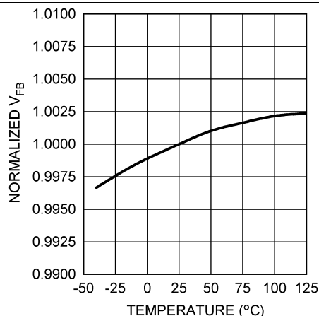
Figure 8. Normalized Feedback Voltage vs Temperature
