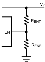
Figure 12. External UVLO Connections
