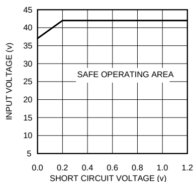
Figure 16. SOA at 300 kHz
