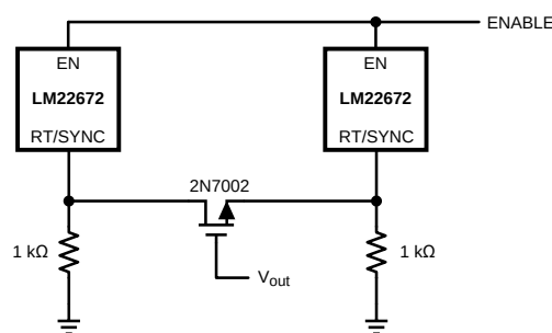
Figure 14. Self-Synchronizing Setup
