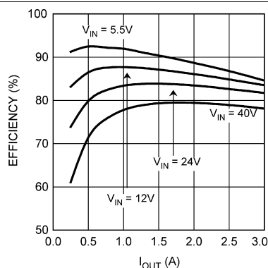
Figure 21. Efficiency vs I_{OUT} and V_{IN} , V_{OUT} = 3.3 V
