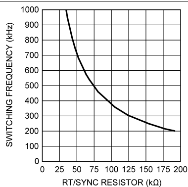
Figure 22. Switching Frequency vs RT/SYNC Resistor
