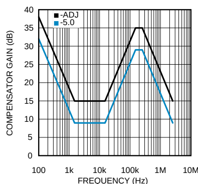
Figure 15. Compensator Gain
