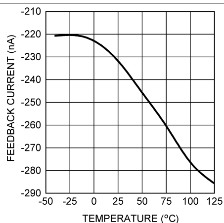
Figure 5. Feedback Bias Current vs Temperature
