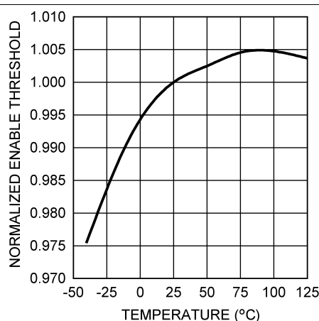
Figure 6. Normalized Enable Threshold Voltage vs Temperature
