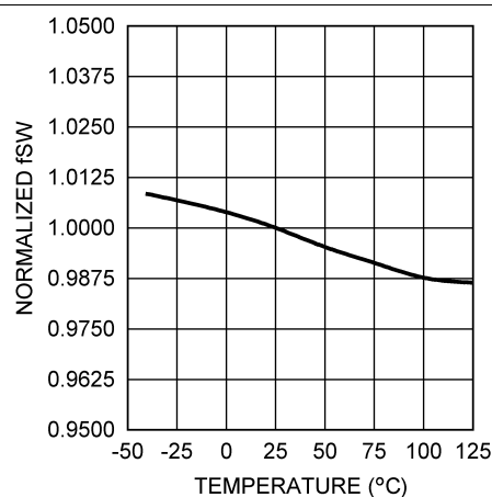
Figure 16. Normalized Switching Frequency vs Temperature
