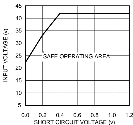
Figure 12. SOA
