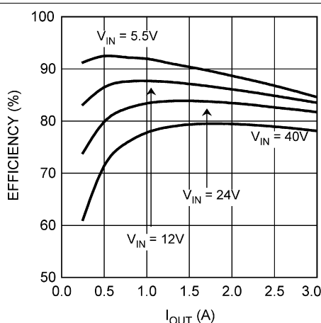
Figure 15. Efficiency vs I_{OUT} and V_{IN} , V_{OUT} = 3.3 V
