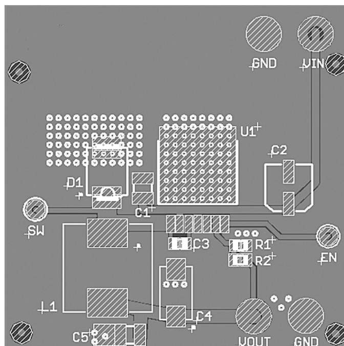
Figure 17. PCB Layout Example for PFM Package
