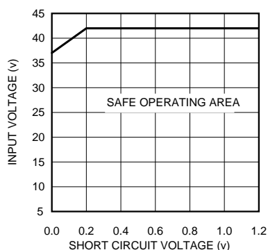
Figure 15. SOA at 300 kHz
