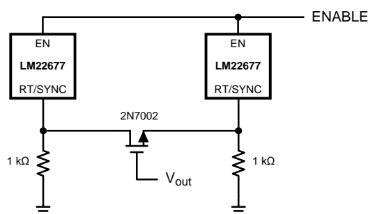
Figure 13. Self Synchronizing Setup
