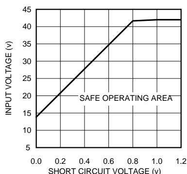
Figure 17. SOA at 800 kHz
