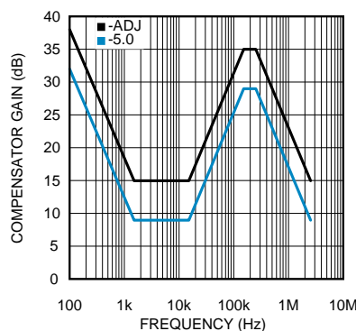
Figure 14. Compensator Gain
