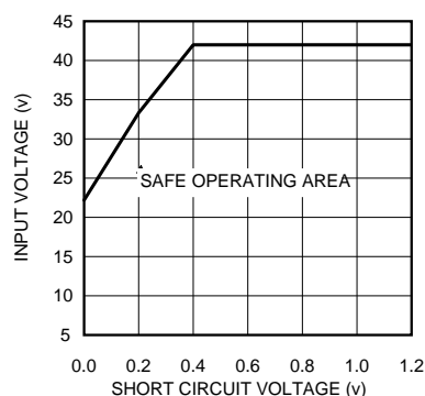
Figure 16. SOA at 500 kHz
