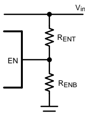
Figure 11. External UVLO Connections
