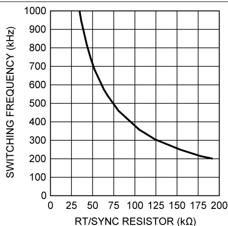
Figure 21. Switching Frequency vs RT/SYNC Resistor
