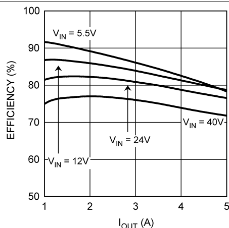
Figure 20. Efficiency vs I_{OUT} and V_{IN} , V_{OUT} = 3.3 V
