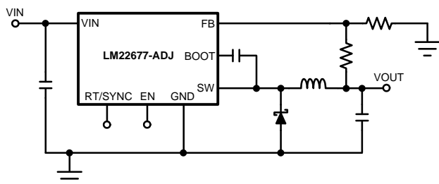
Simplified Application Schematic
