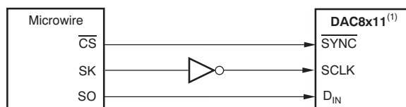
Figure 82. DAC8x11 to Microwire Interface
