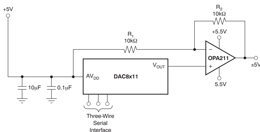
Figure 89. Bipolar Operation With the DAC8x11
