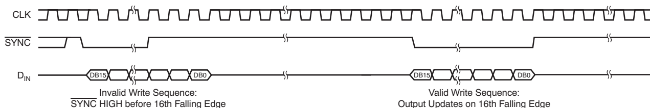
Figure 78. DAC8311 \overline{\text{SYNC}} Interrupt Facility
