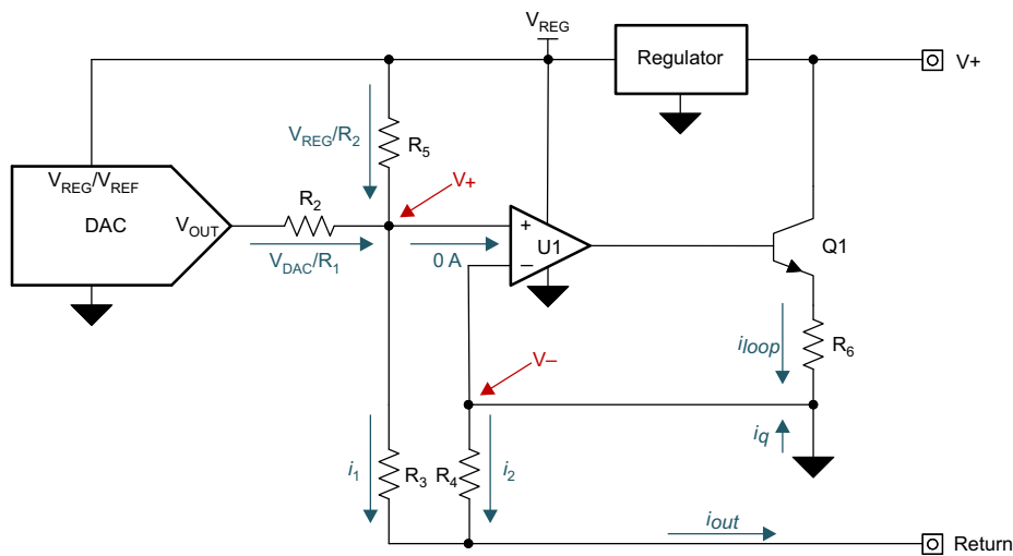
Figure 85. Voltage to Current Conversion
