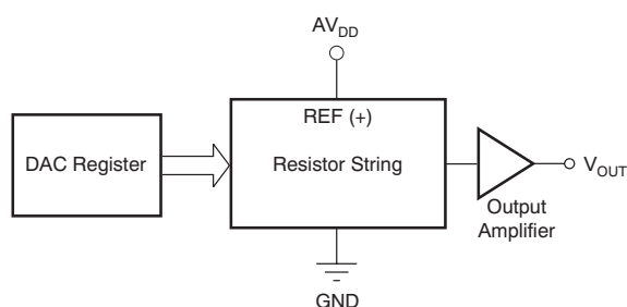
Figure 74. DAC8x11 Architecture
