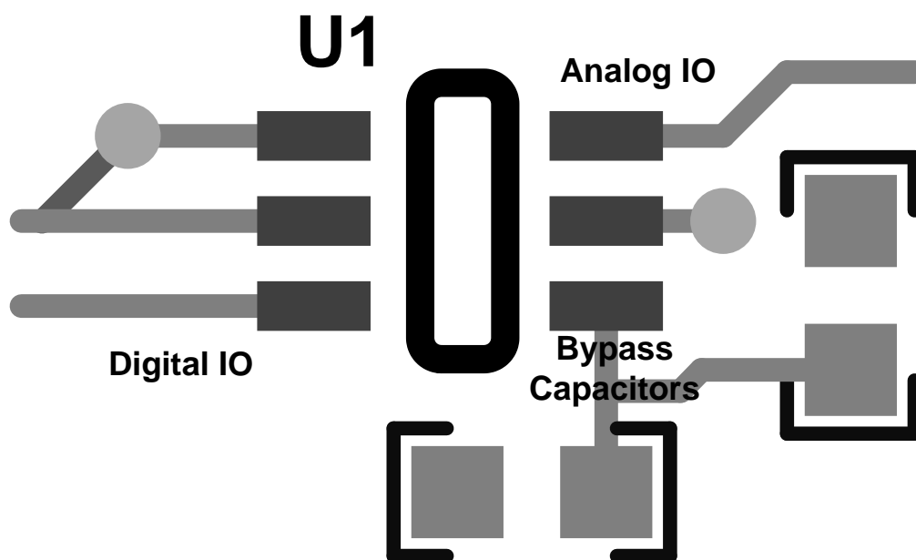
Figure 90. Recommended Layout
