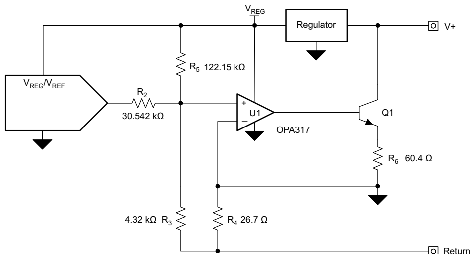
Figure 84. Loop Powered Transmitter Schematic
