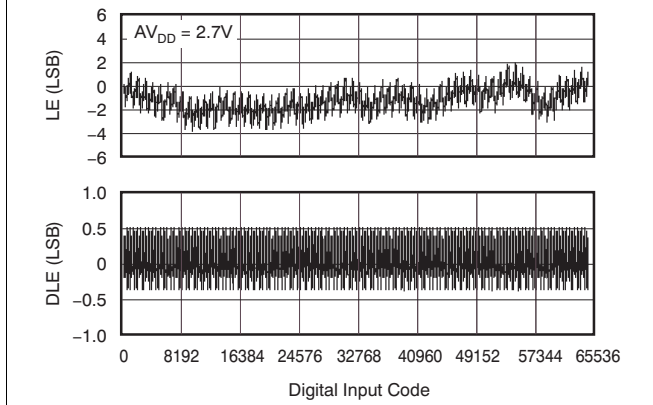
Figure 46. DAC8411 16-Bit Linearity Error and Differential Linearity Error vs Code (25°C)
