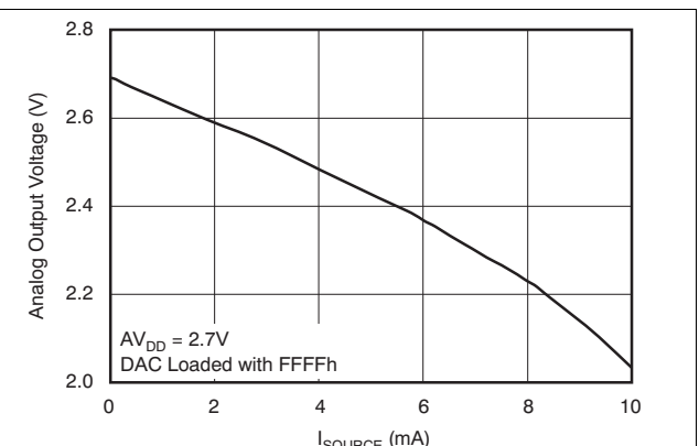
Figure 51. Source Current at Positive Rail
