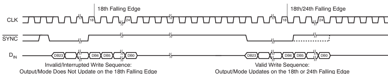
Figure 80. DAC8411 \overline{\text{SYNC}} Interrupt Facility
