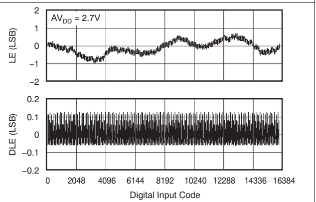
Figure 47. DAC8311 14-Bit Linearity Error and Differential Linearity Error vs Code (25°C)
