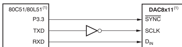
Figure 81. DAC8x11 to 80C51/80L51 Interfaces
