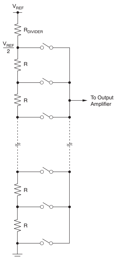
Figure 75. Resistor String
