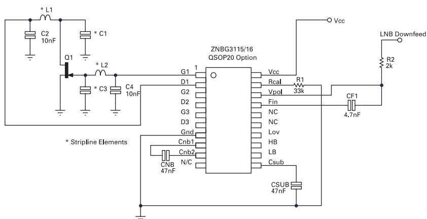
QSOP20 Applications circuit
