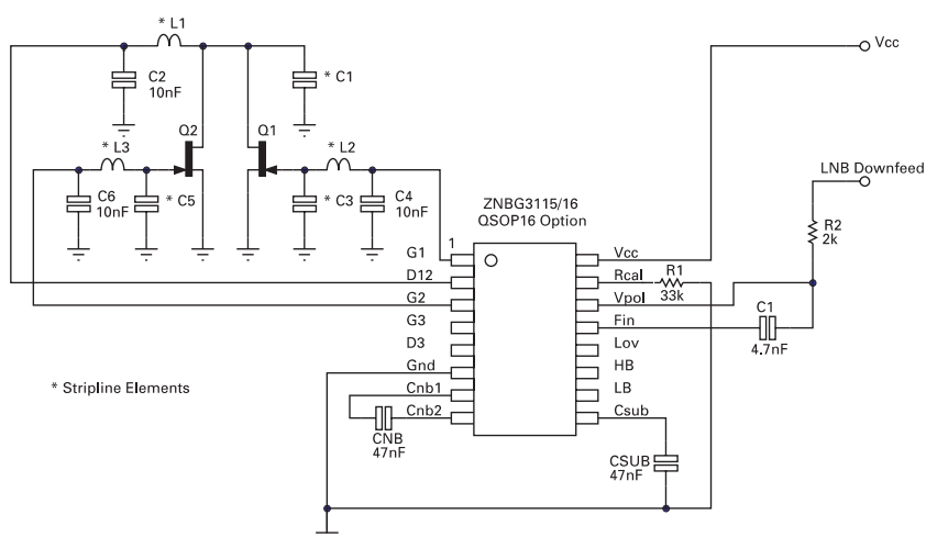
QSOP16 Applications circuit
