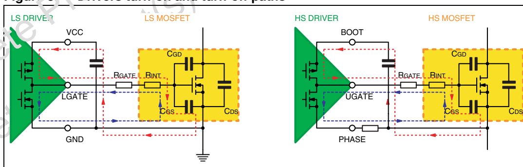
Figure 3 Drivers turn-on and turn-off paths
