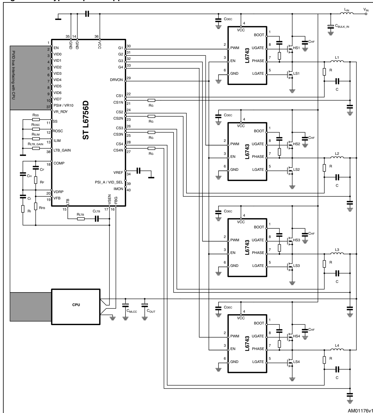
Figure 1. Typical 4phase application circuit
