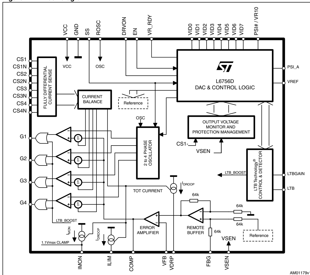
Figure 4. Block diagram
