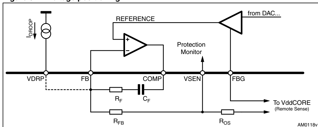
Figure 6. Voltage positioning
