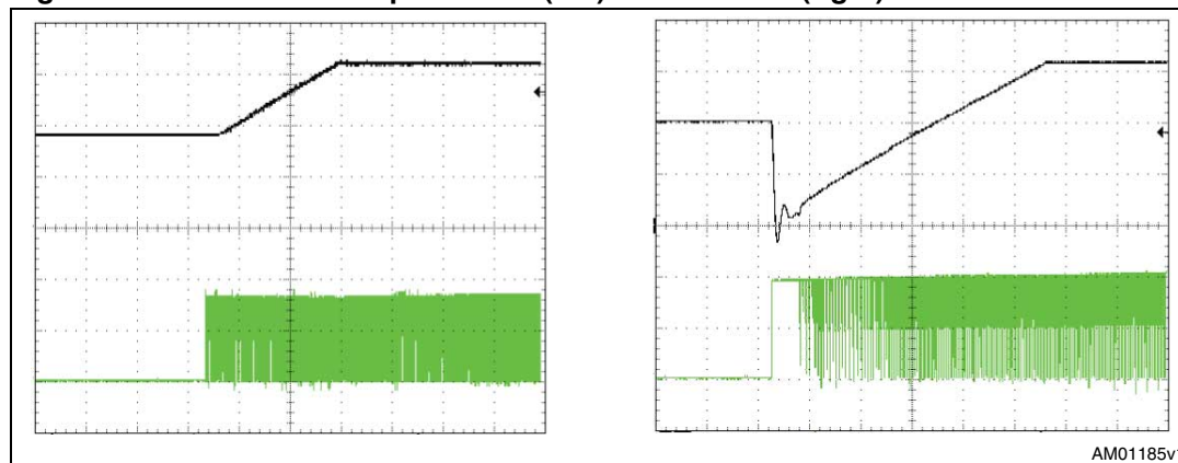
Figure 10. LSLESS start-up: enabled (left) and disabled (right)
