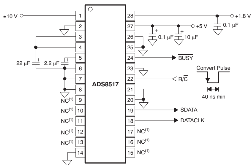
Figure 29. Basic \pm 10 -V Operation with Serial Output
