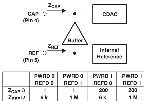
Figure 41. Characteristic Impedances of the Internal Buffer
