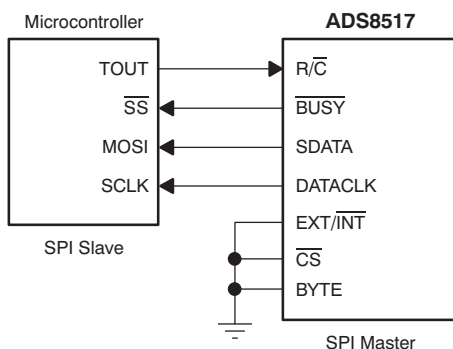
Figure 44. ADS8517 as SPI Master
