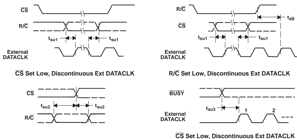
Figure 32. Critical Timing Parameters
