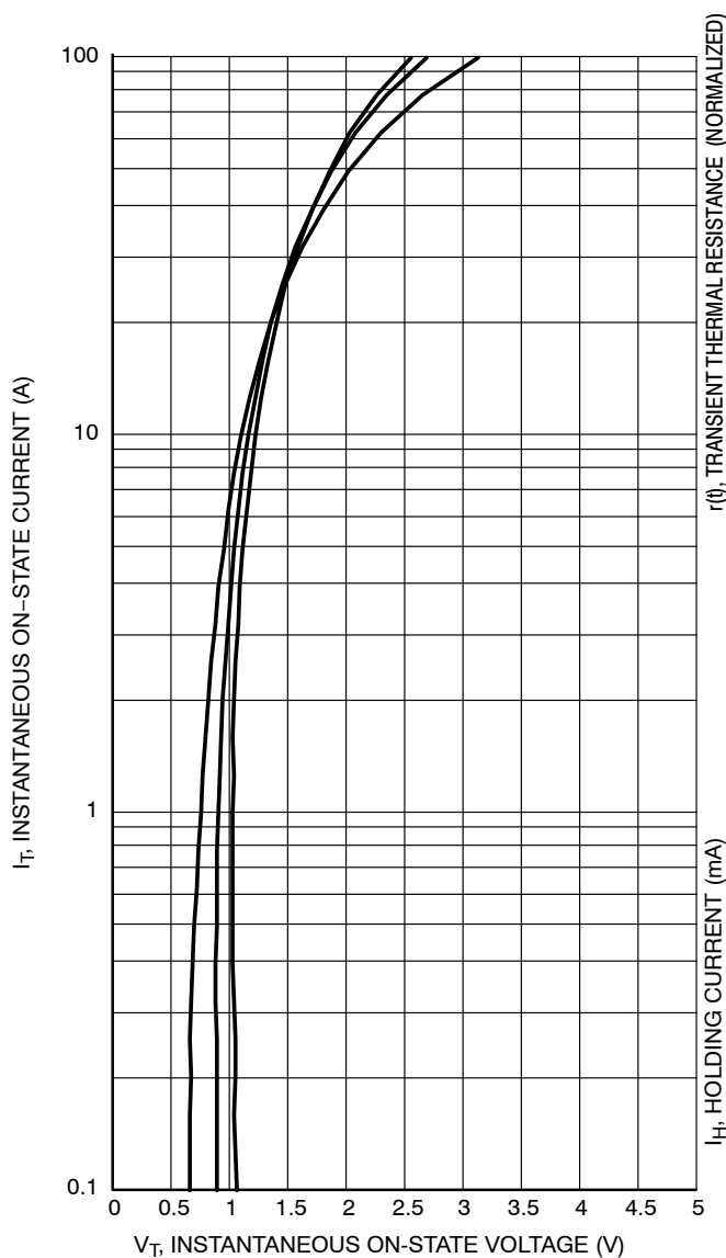
Figure 3. On-State Characteristics
