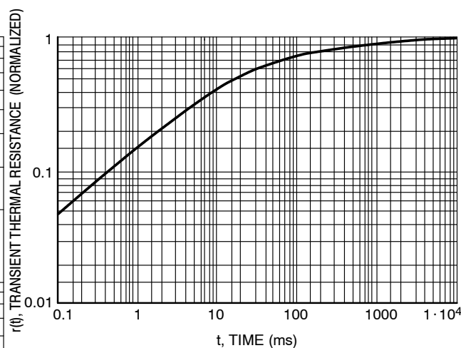
Figure 4. Thermal Response
