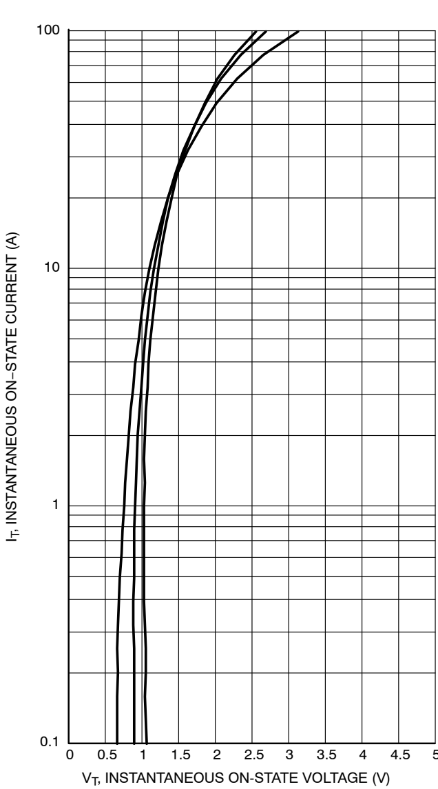
Figure 3. On-State Characteristics
