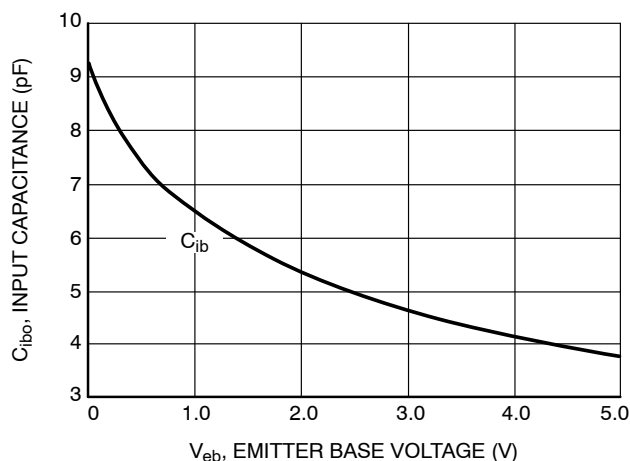
Figure 6. Input Capacitance
