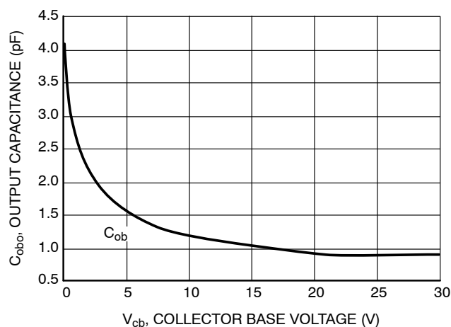
Figure 7. Output Capacitance
