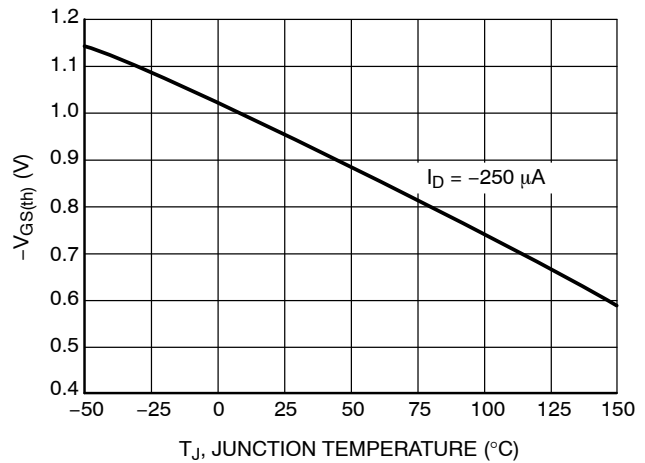
Figure 10. Threshold Voltage
