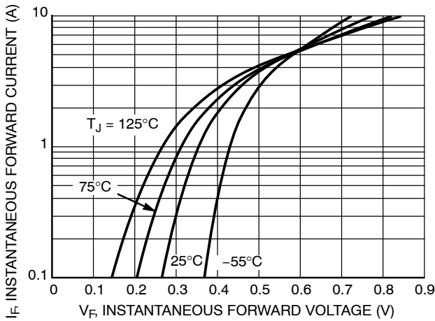
Figure 14. Typical Forward Voltage
