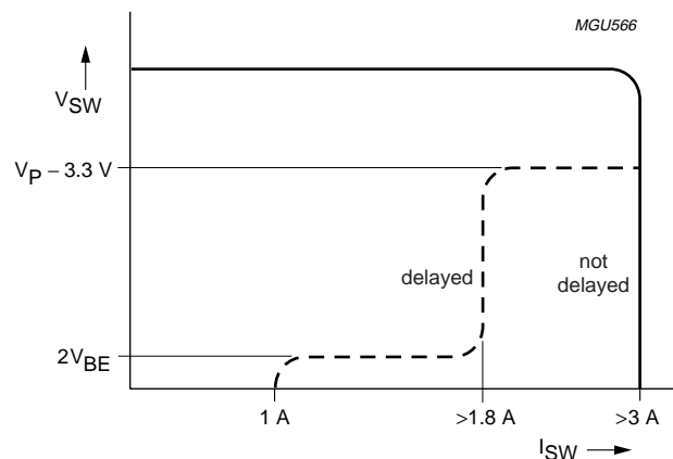
Fig.7 Current protection of the power switch.
