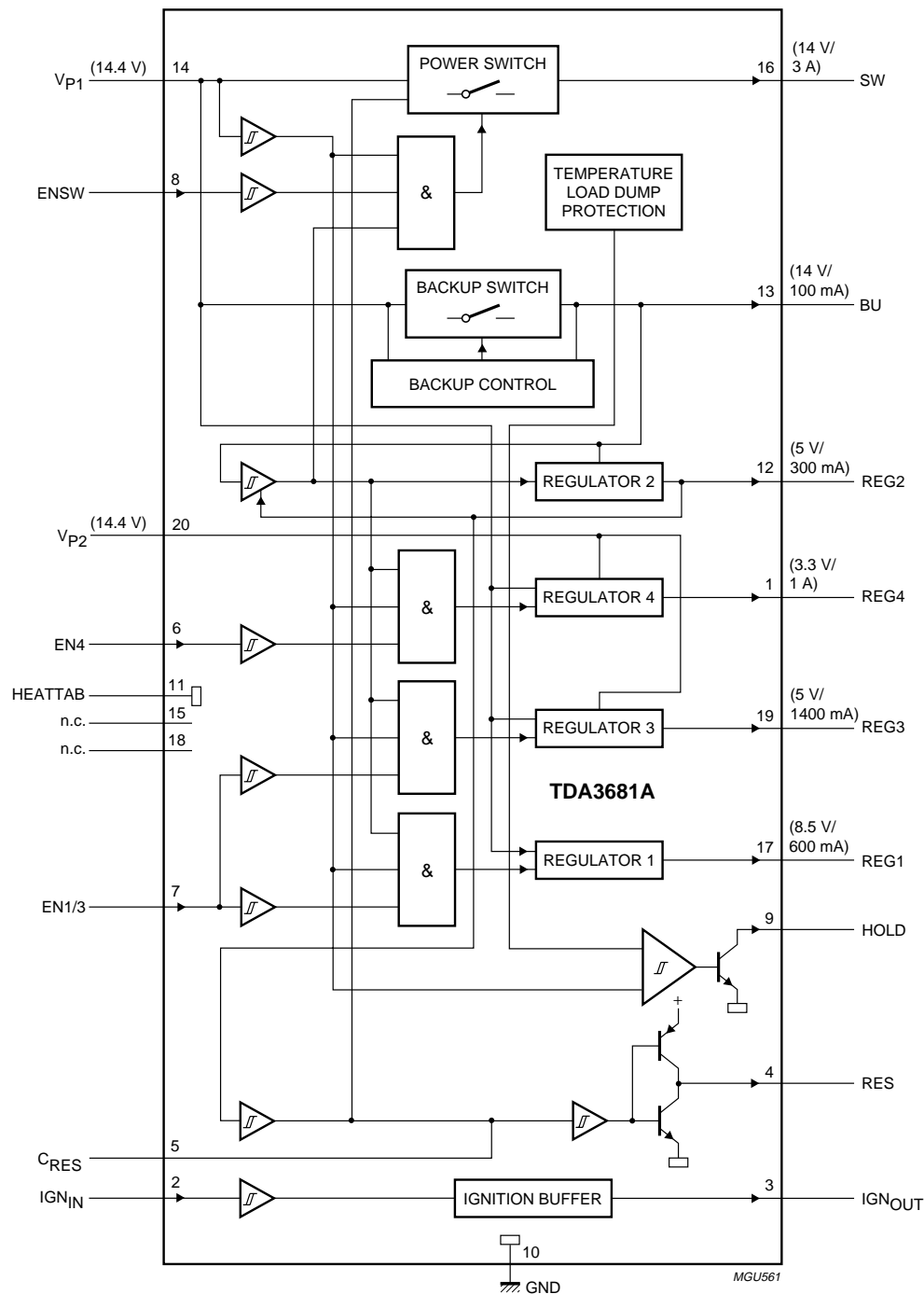
Fig.1 Block diagram.
