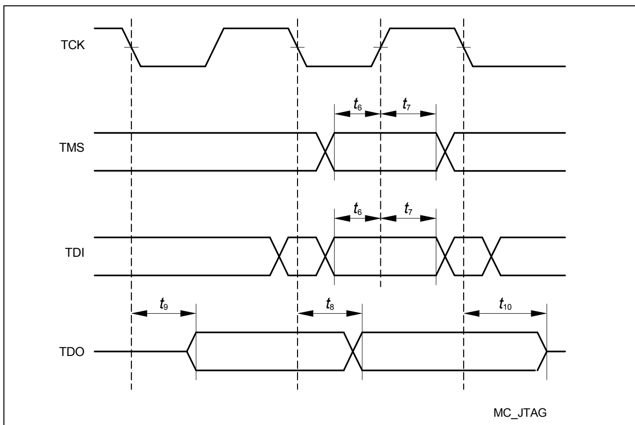
Figure 27 JTAG Timing
