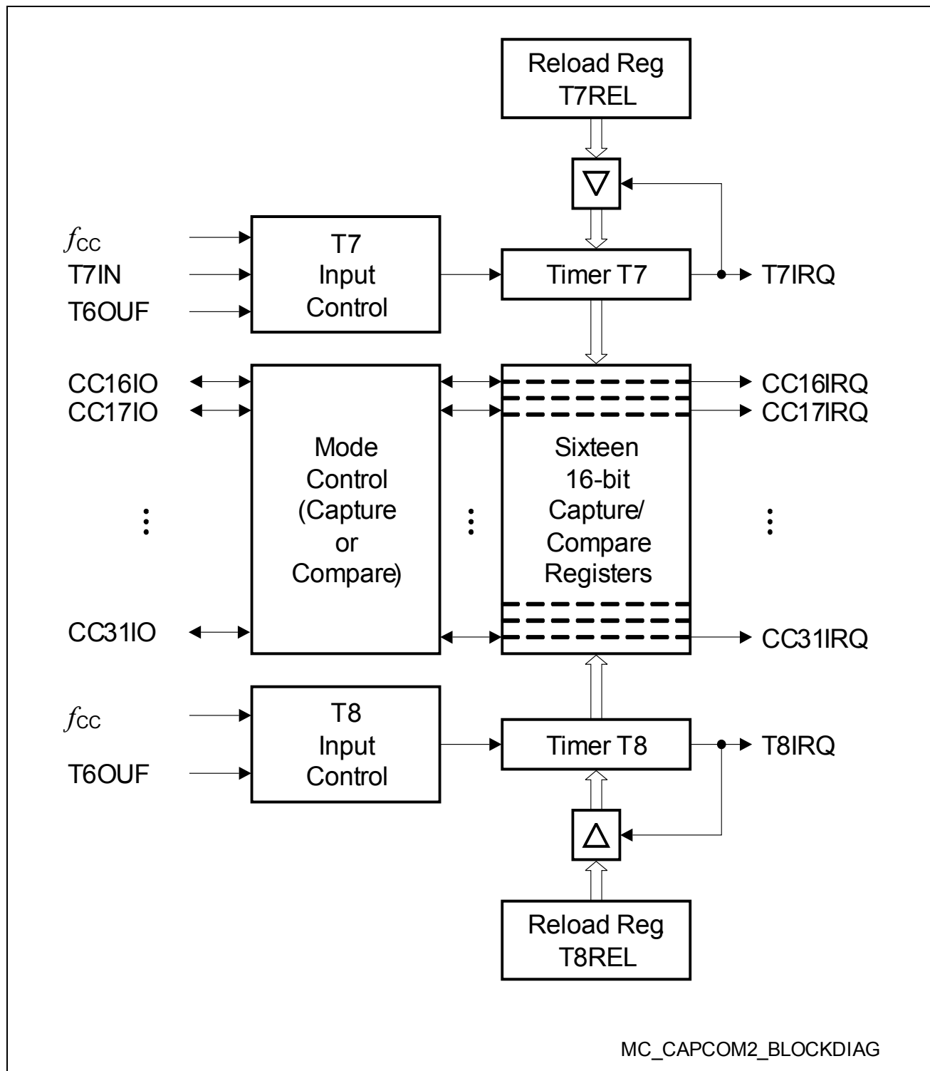
Figure 5 CAPCOM2 Unit Block Diagram
