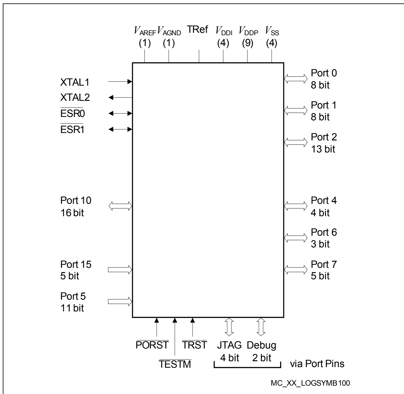
Figure 1 Logic Symbol
