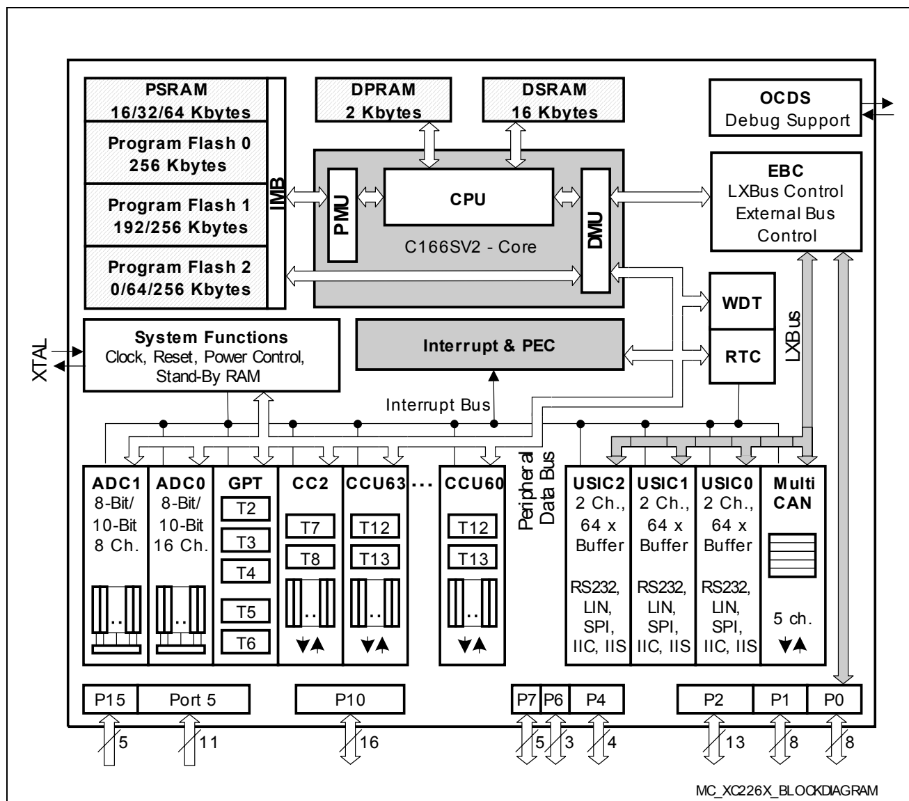
Figure 3 Block Diagram
