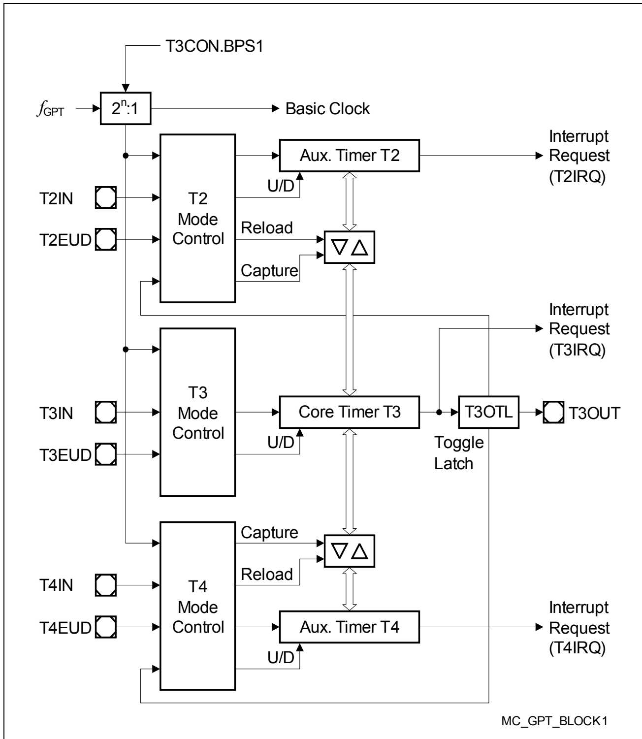
Figure 7 Block Diagram of GPT1
