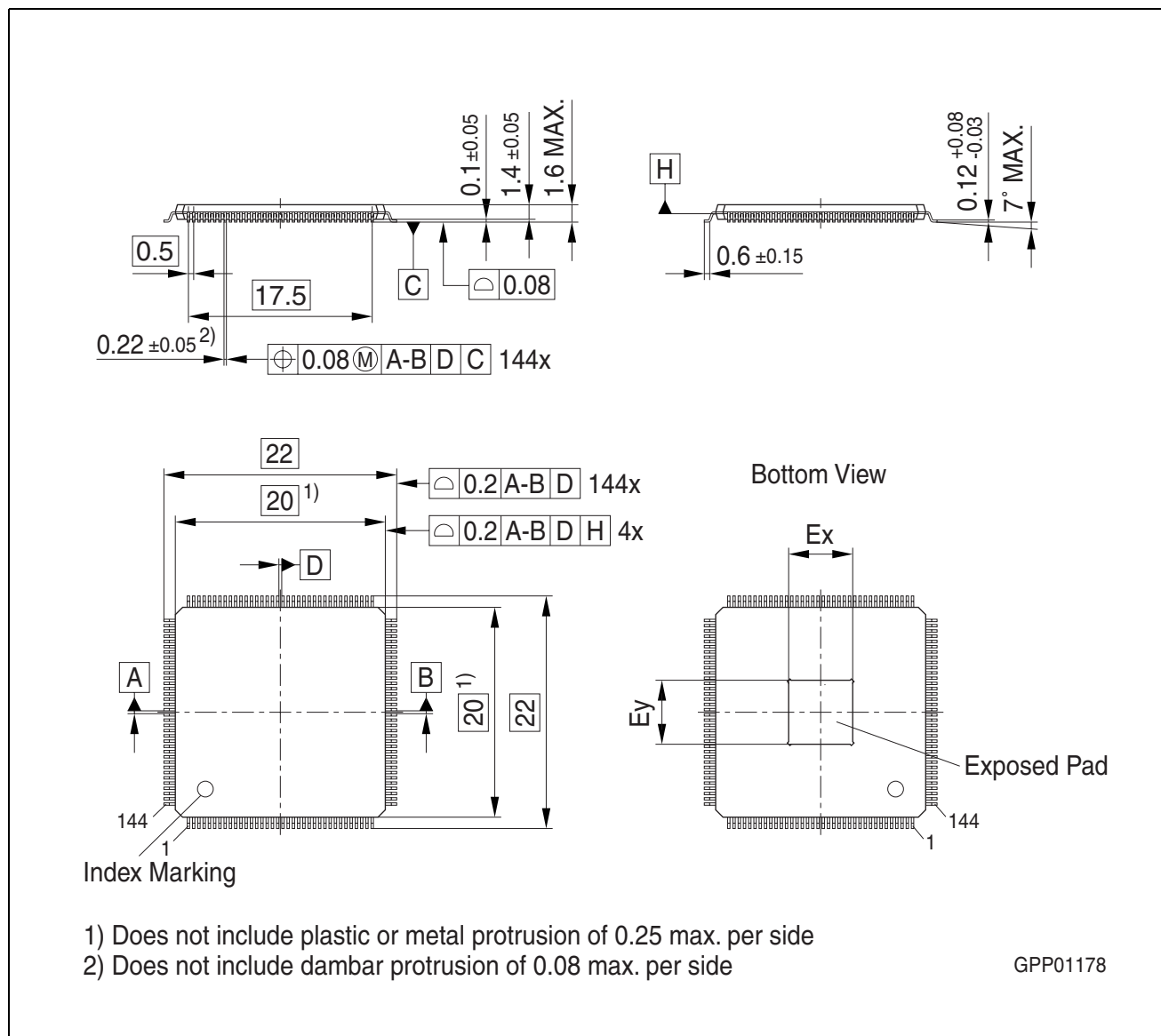
Figure 30 PG-LQFP-144-4 (Plastic Green Thin Quad Flat Package)
