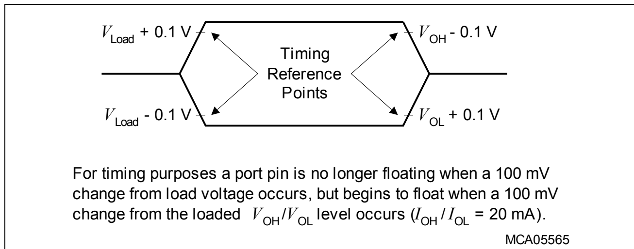
Figure 17 Floating Waveforms
