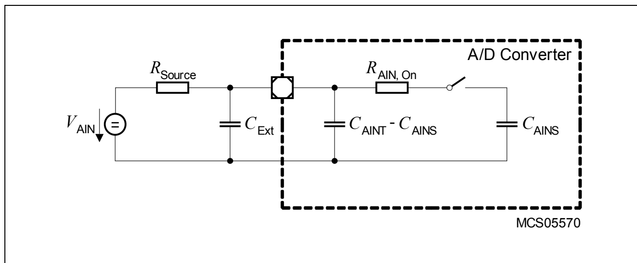
Figure 15 Equivalent Circuitry for Analog Inputs
