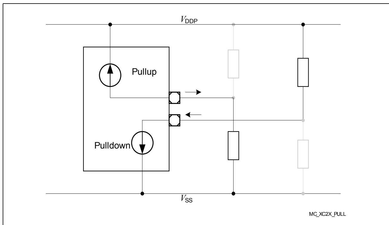
Figure 12 Pullup/Pulldown Current Definition
