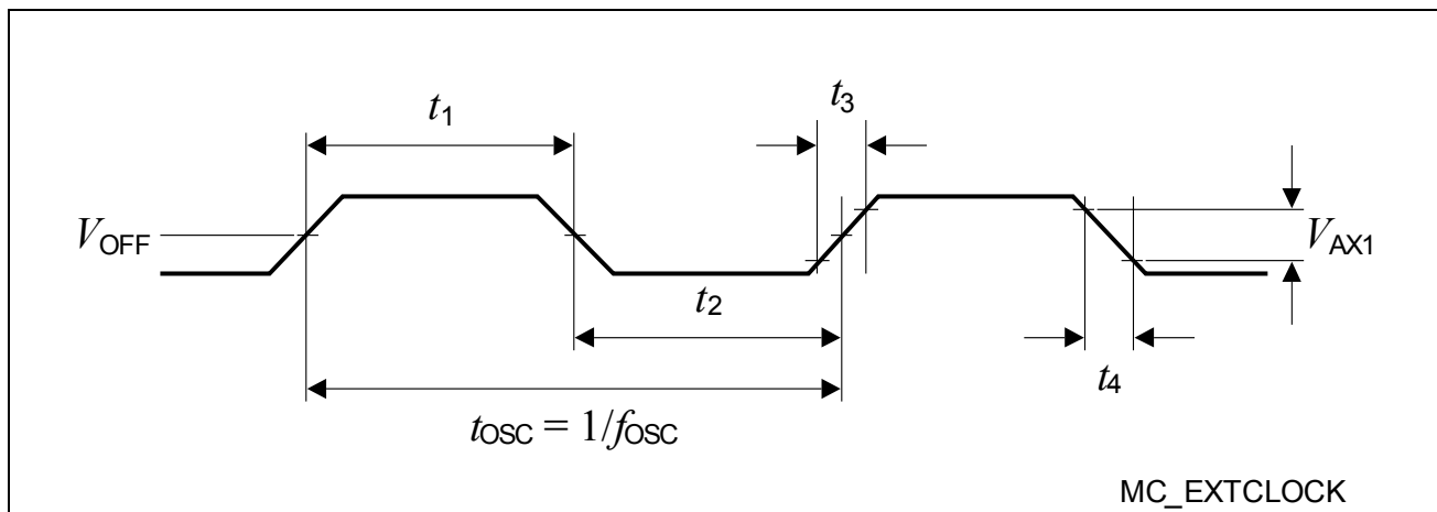
Figure 20 External Clock Drive XTAL1
