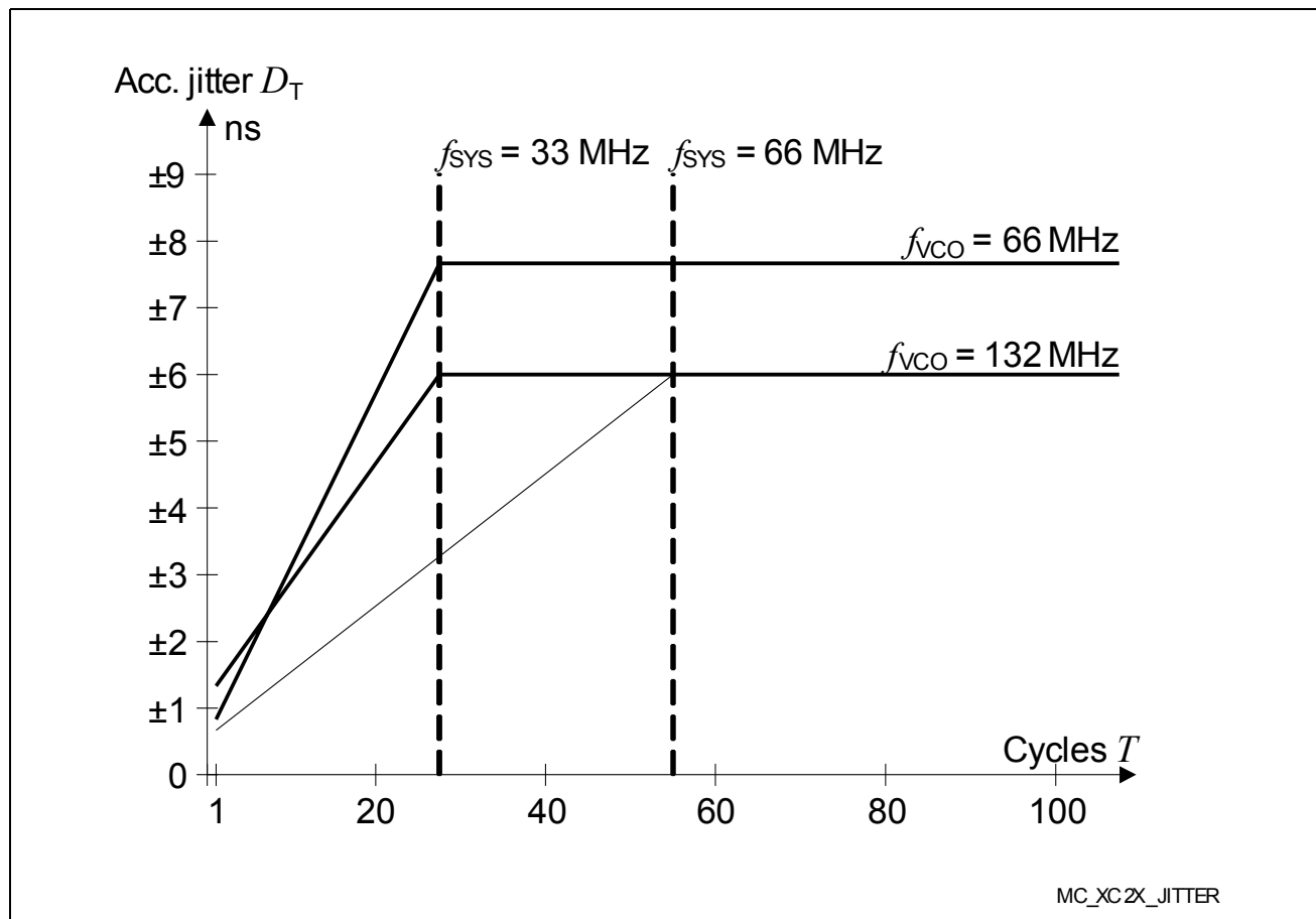
Figure 19 Approximated Accumulated PLL Jitter
