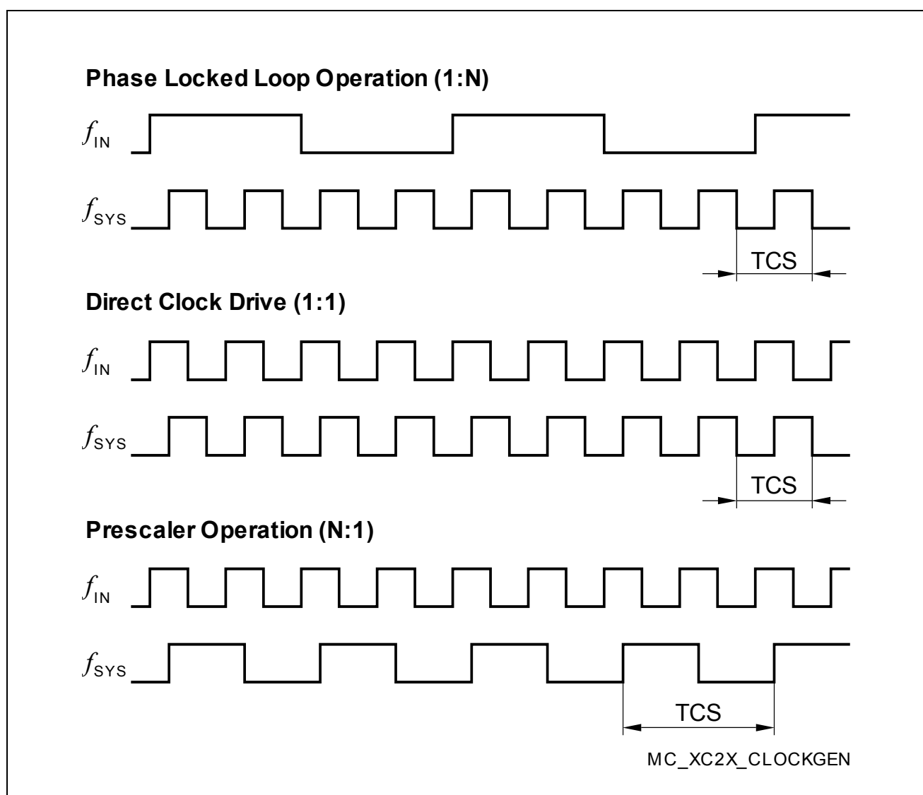
Figure 18 Generation Mechanisms for the System Clock
