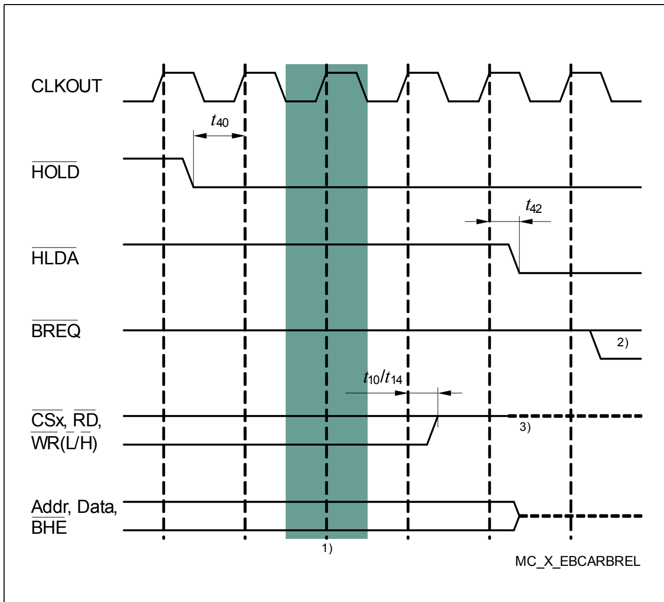
Figure 25 External Bus Arbitration, Releasing the Bus
