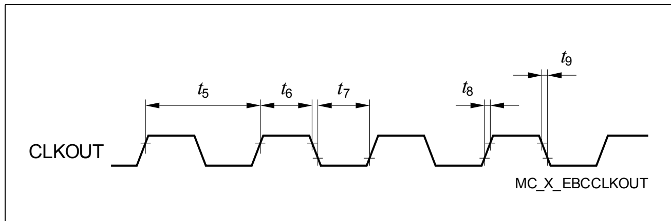
Figure 21 CLKOUT Signal Timing
