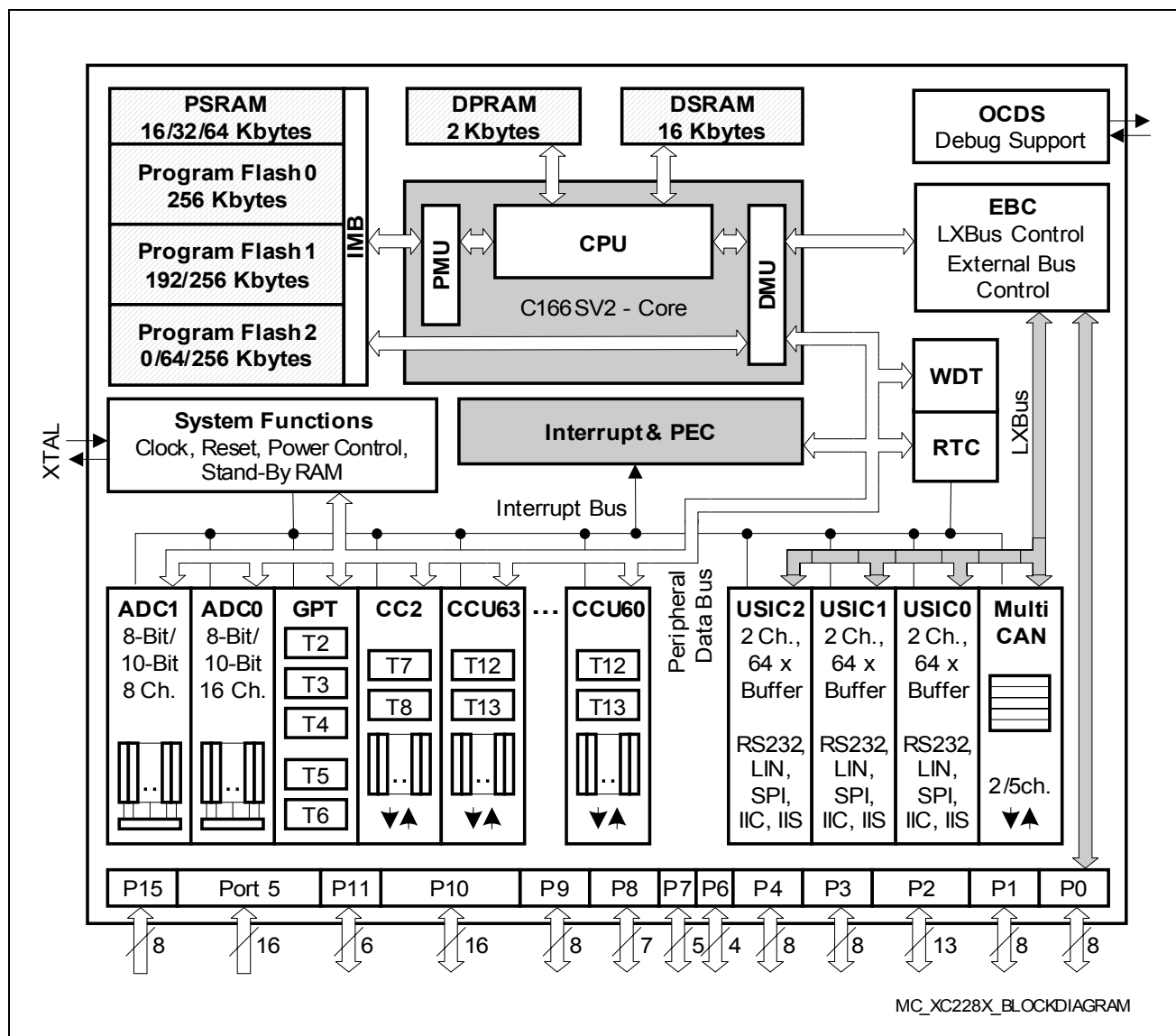
Figure 3 Block Diagram
