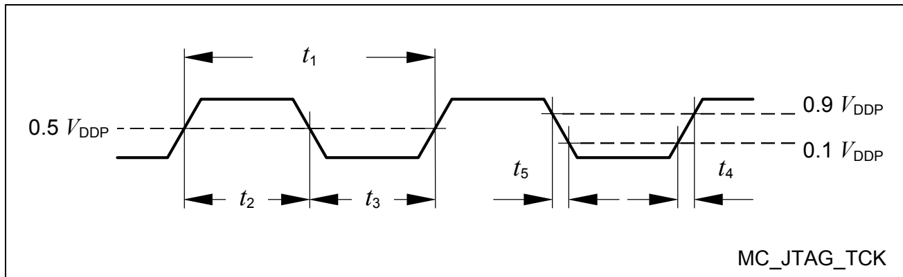
Figure 28 Test Clock Timing (TCK)
