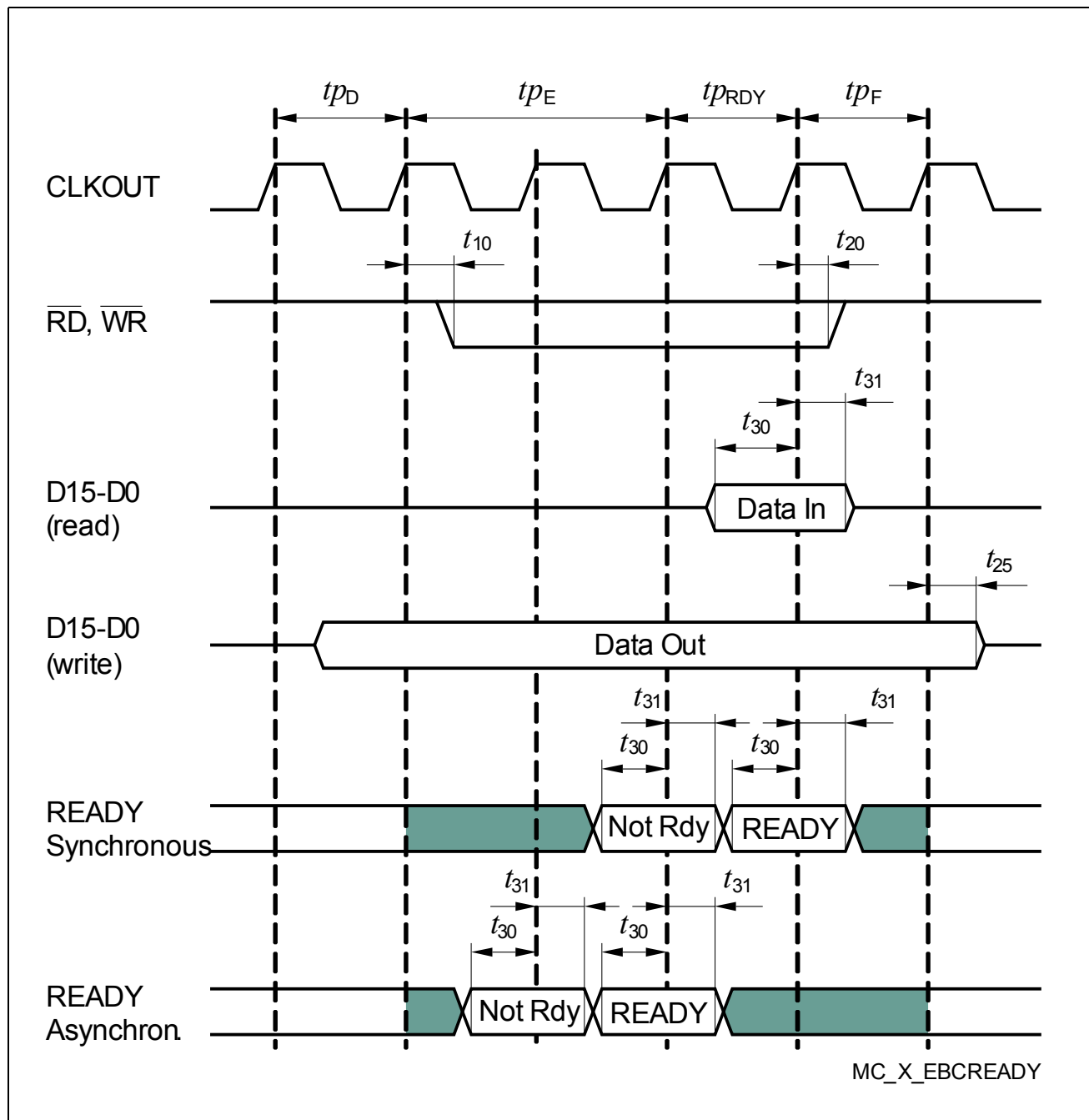
Figure 24 READY Timing
