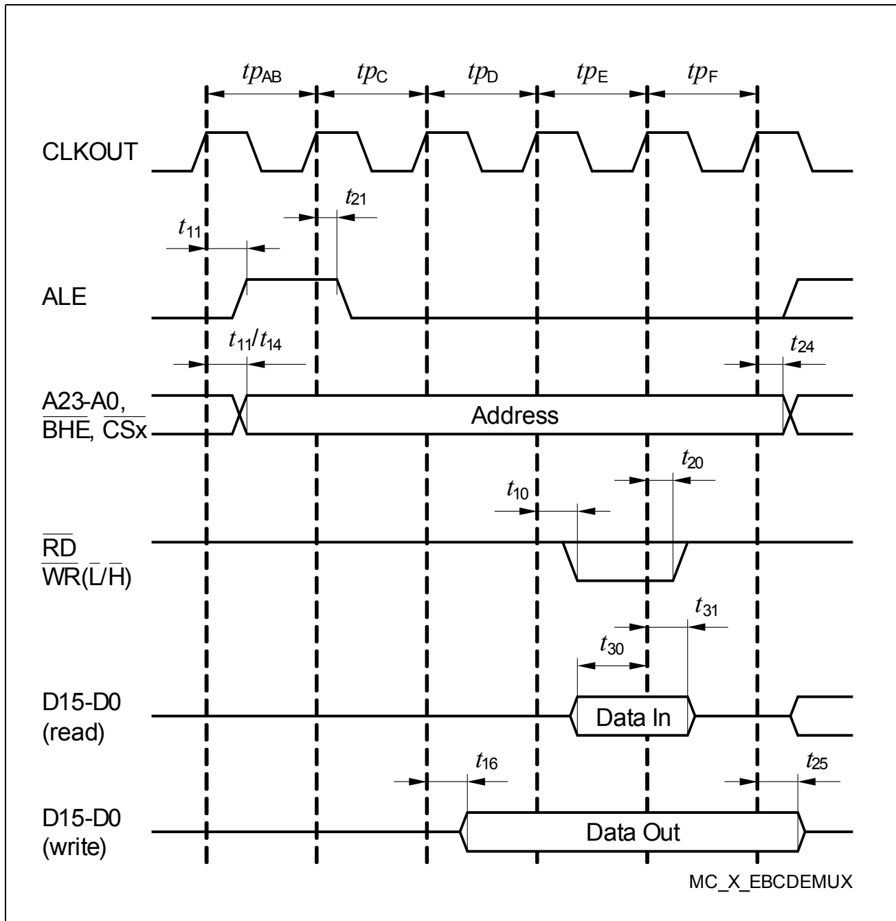
Figure 23 Demultiplexed Bus Cycle
