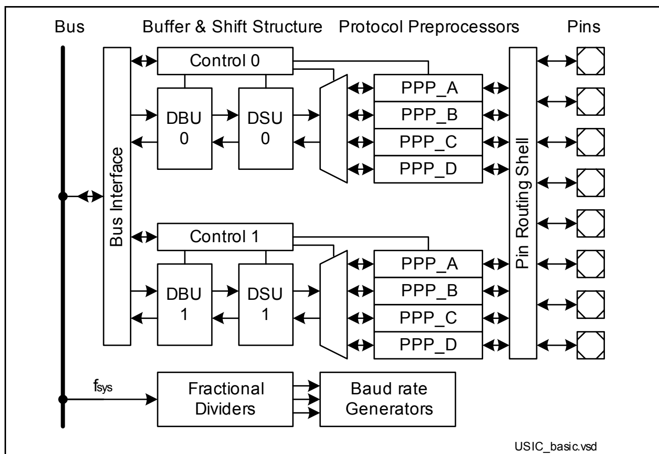
Figure 10 General Structure of a USIC Module
