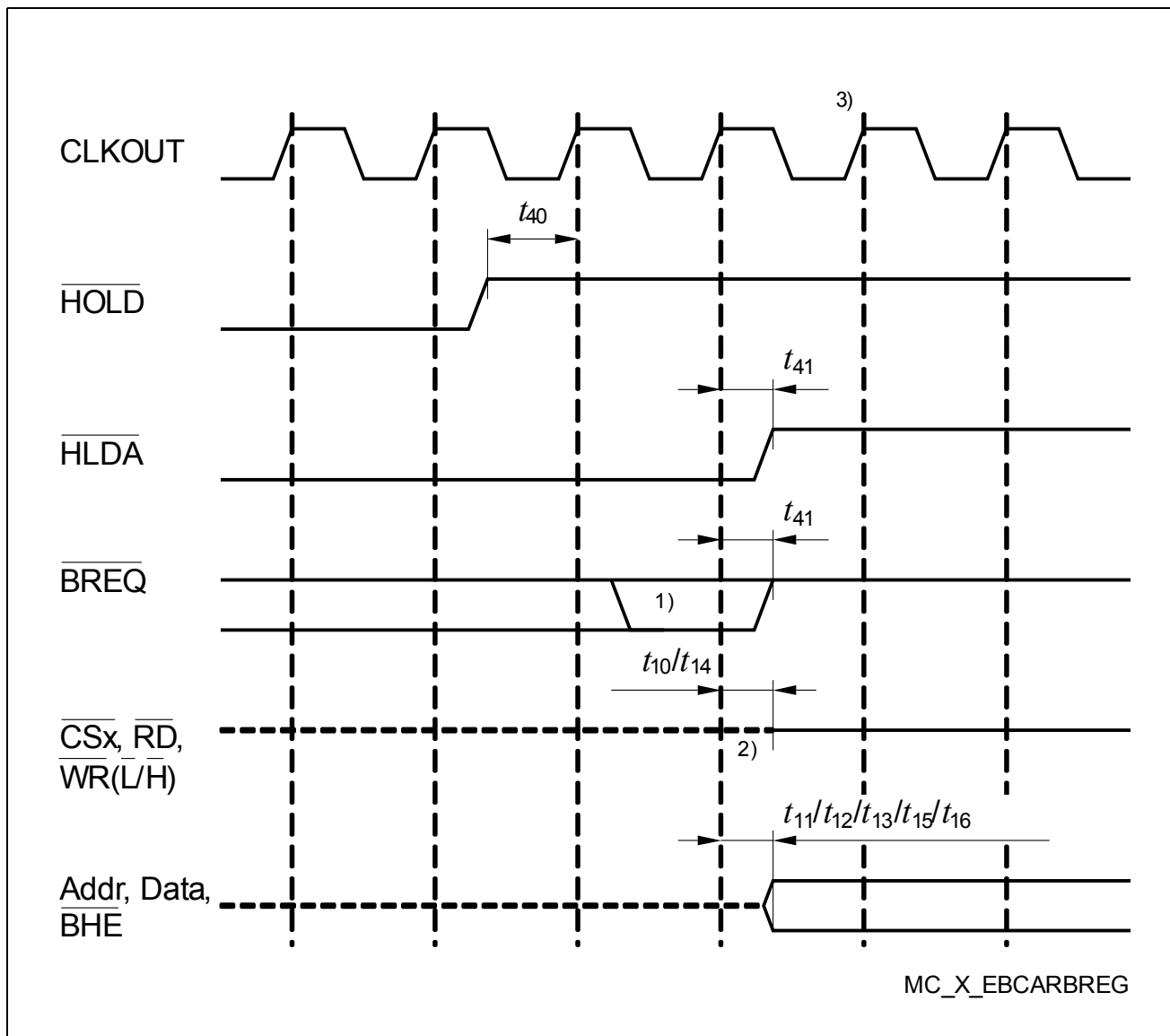
Figure 26 External Bus Arbitration, Regaining the Bus
