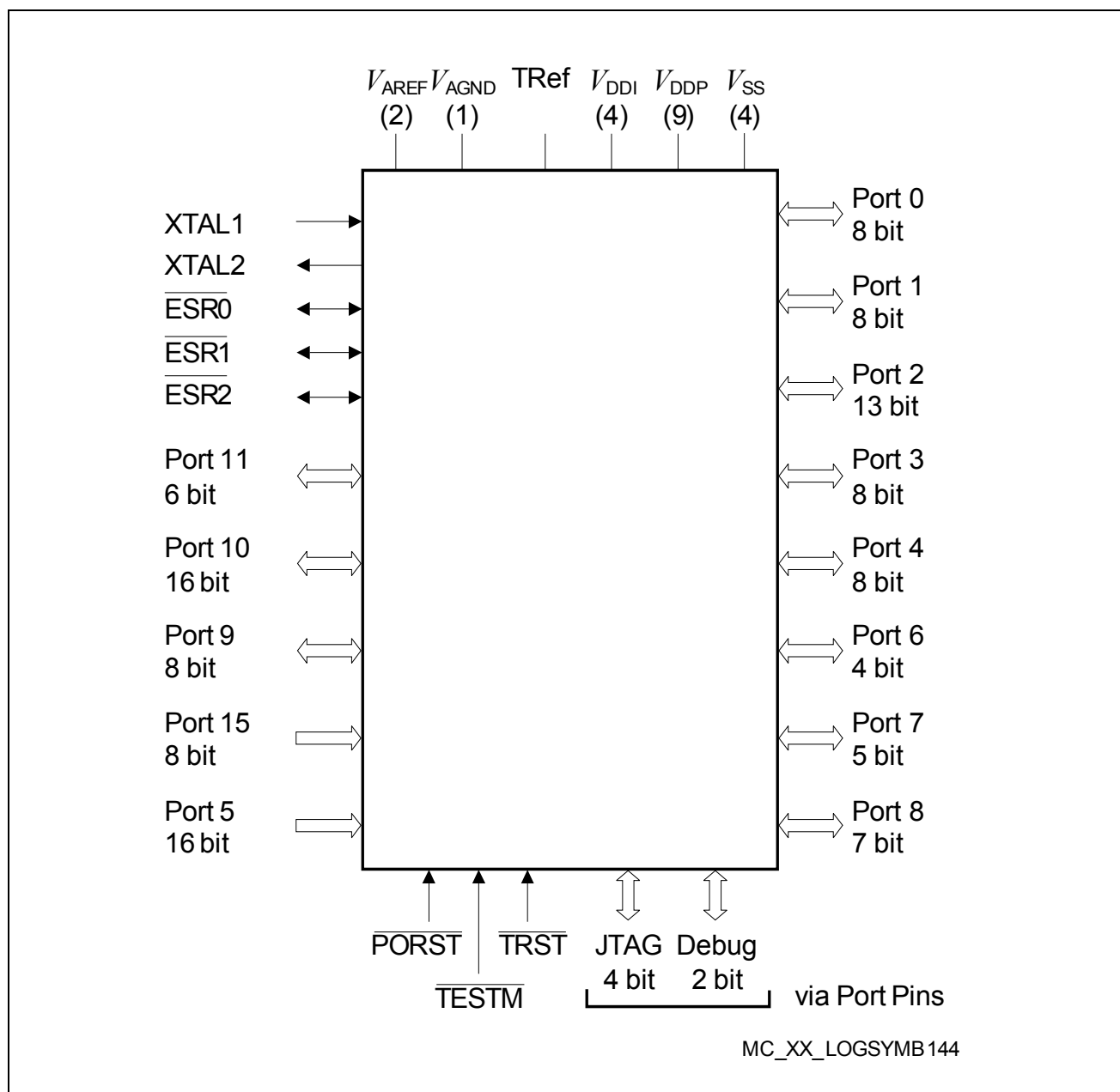
Figure 1 Logic Symbol
