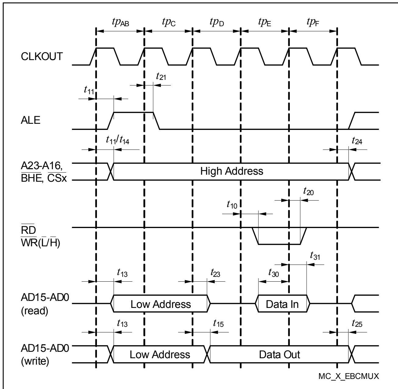
Figure 22 Multiplexed Bus Cycle
