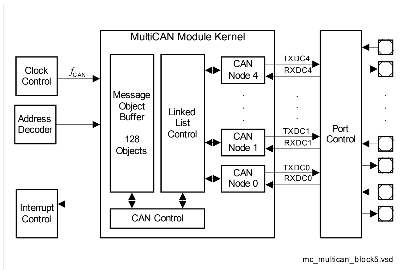
Figure 11 Block Diagram of MultiCAN Module
