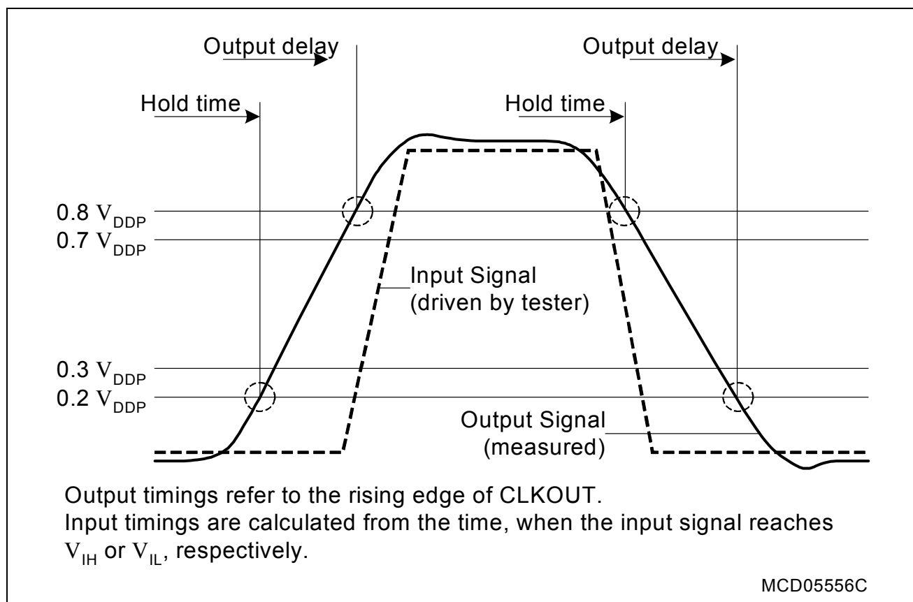
Figure 16 Input Output Waveforms
