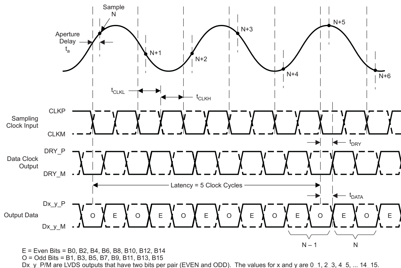
Figure 1. Timing Diagram
