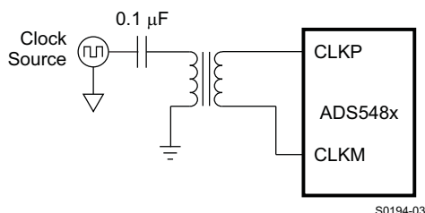
Figure 41. Differential Clock
