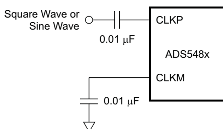
Figure 38. Single-Ended Clock
