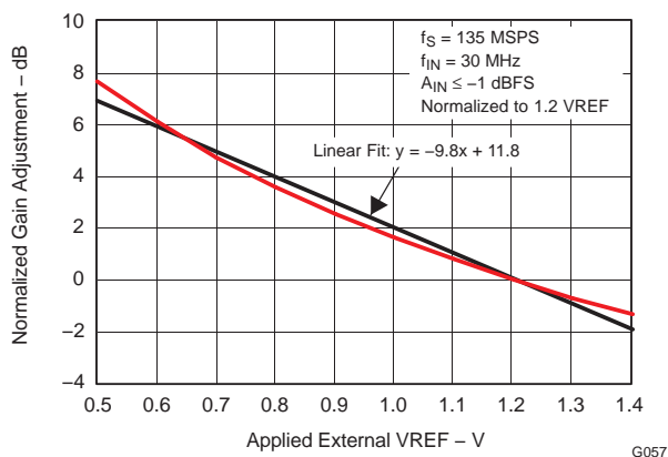
Figure 32. Signal Gain Adjustment versus External Reference (VREF)
