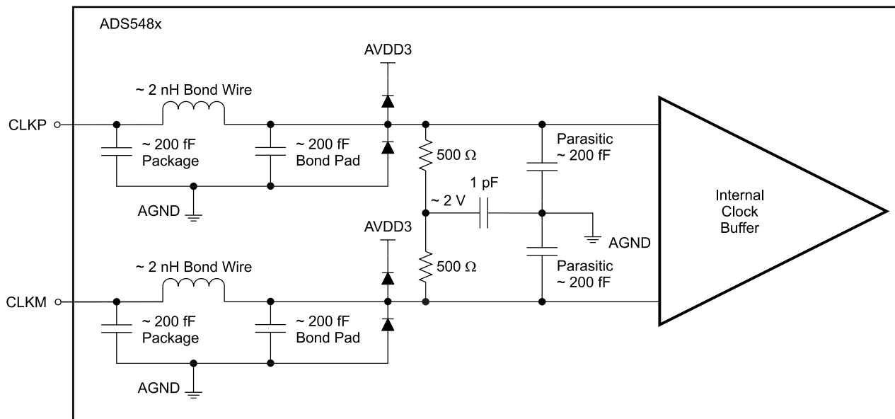
Figure 37. Clock Input Circuit
