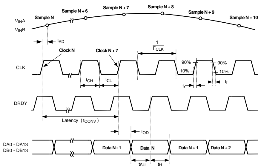
Figure 1. Output Timing
