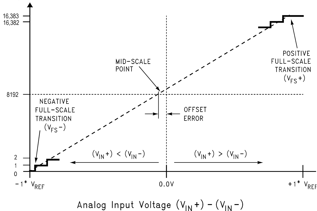
Figure 2. Transfer Characteristic
