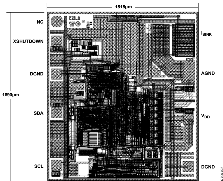
Figure 4. Metallization Photo Dimensions shown in microns (μm)
