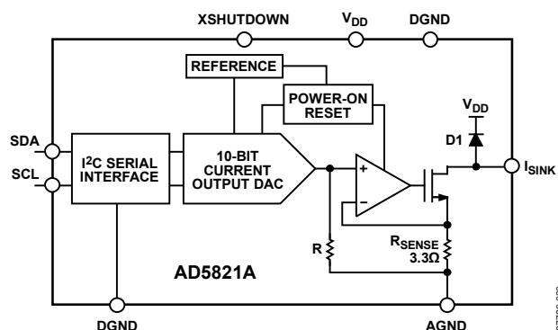
Figure 20. Block Diagram Showing Connection to Voice Coil
