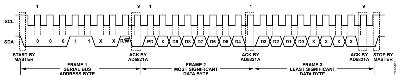
Figure 23. Read Operation
