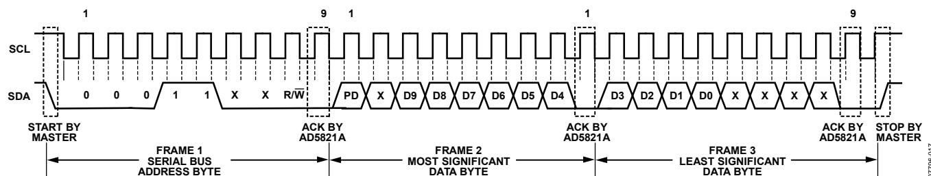
Figure 22. Write Operation
