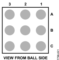
Figure 3. Pin Configuration
