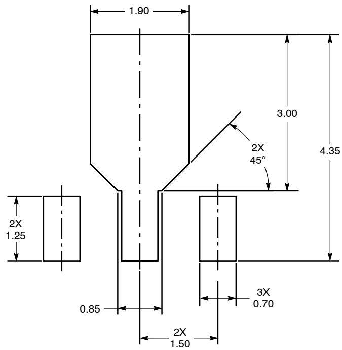
Figure 26. PCB Pad Layout for SOT-89A
