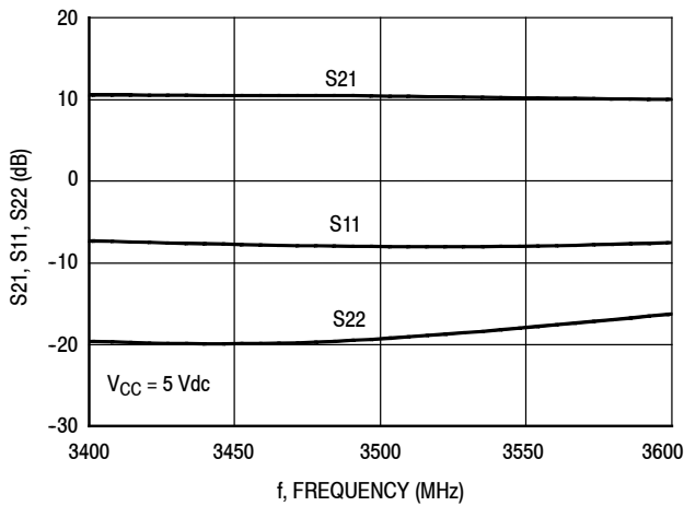
Figure 24. S21, S11 and S22 versus Frequency
