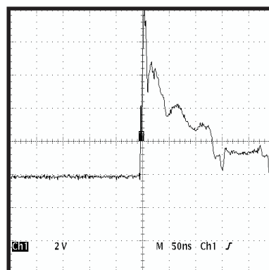
Fig. 6 - ESD Clamping (8kv Contant per IEC 61000-4-2)
