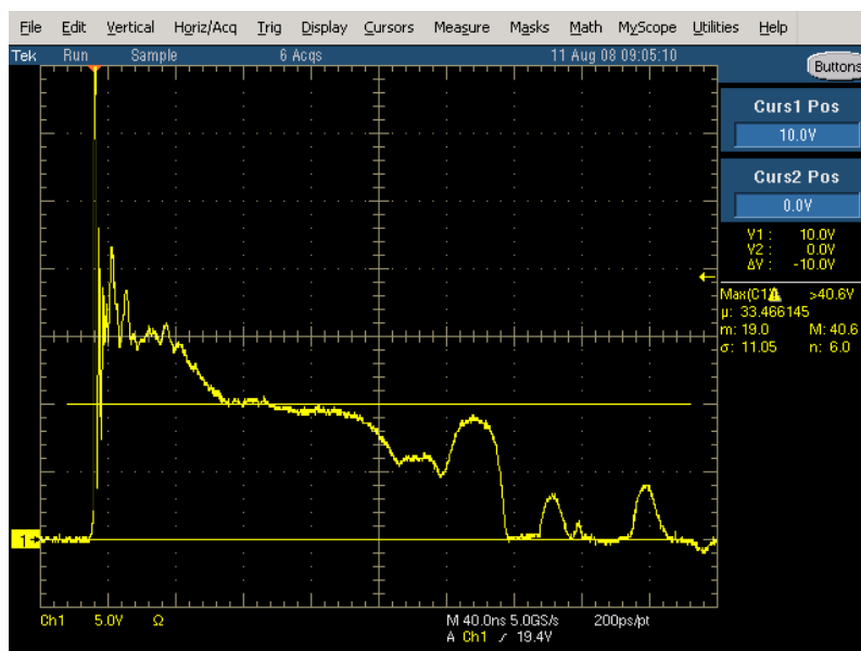
Figure 1. ESD Clamping Voltage Screenshot (8 kV Contact per IEC610000-4-2)
