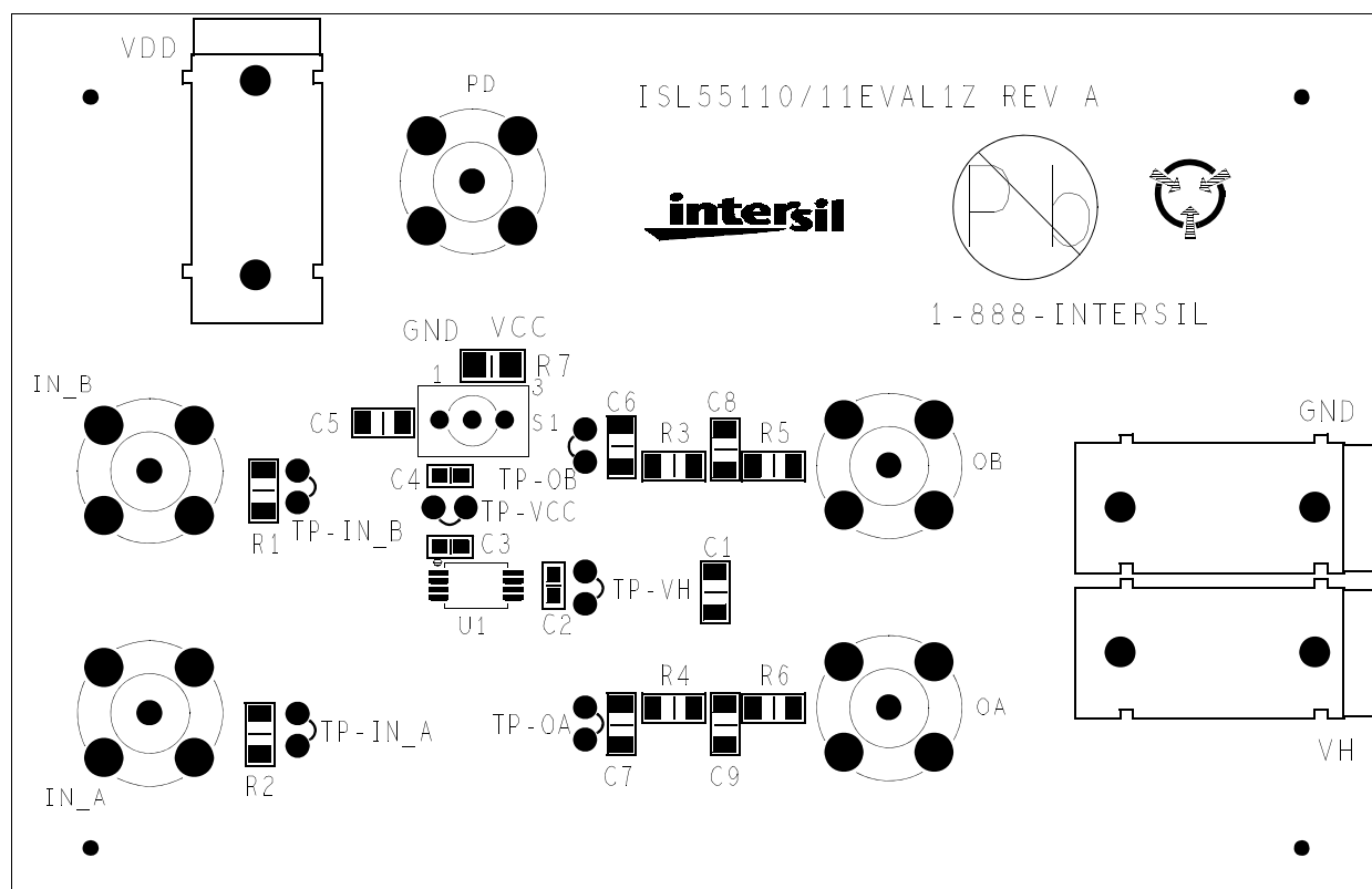
FIGURE 6. TSSOP LAYOUT
