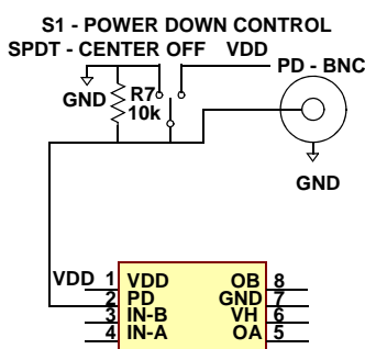
ISL55110, ISL55111_TSSOP
