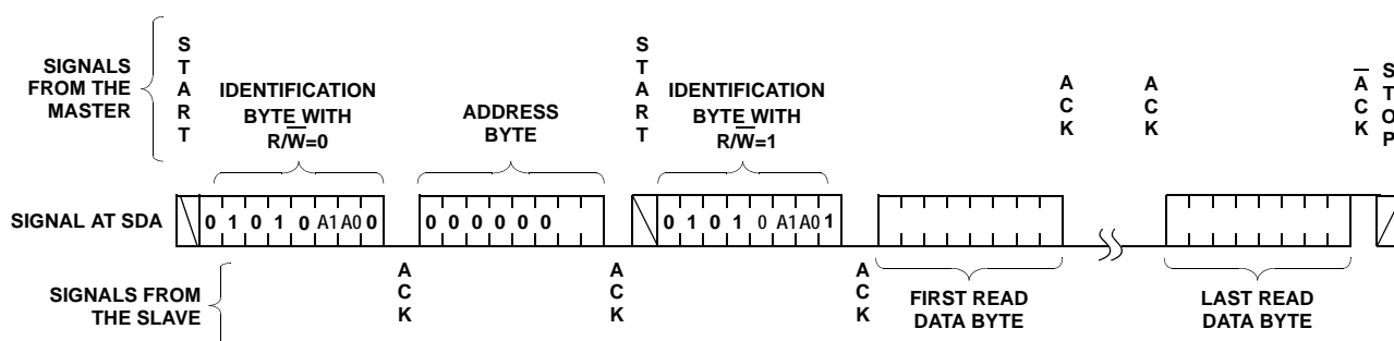
FIGURE 14. READ SEQUENCE
