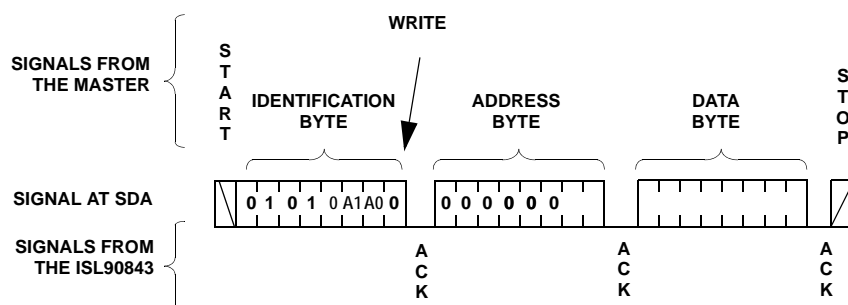
FIGURE 13. BYTE WRITE SEQUENCE
