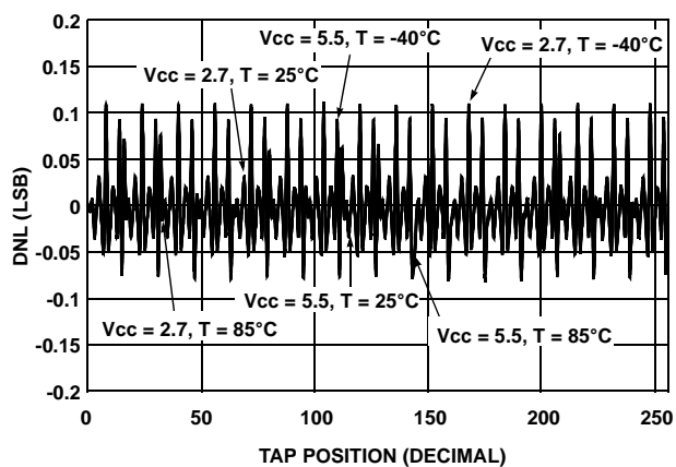
FIGURE 3. DNL vs TAP POSITION FOR 10kΩ (W)
