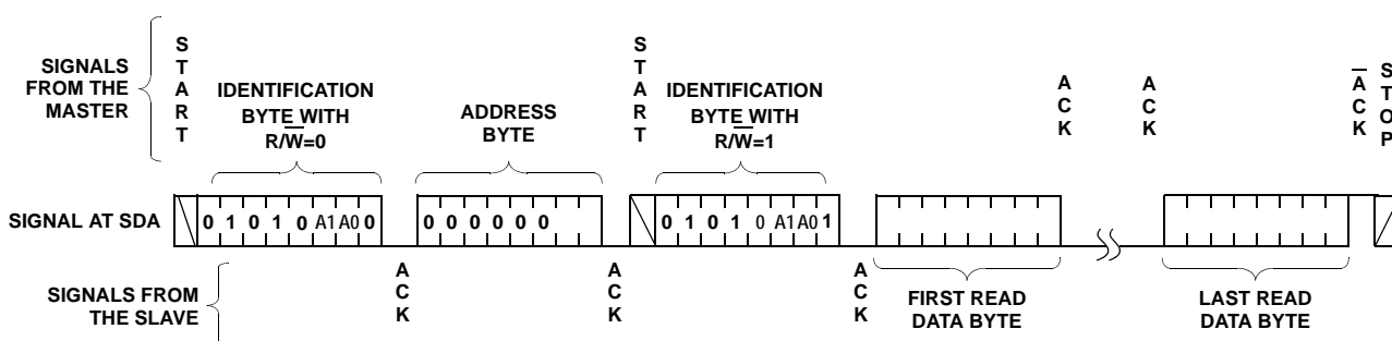
FIGURE 14. READ SEQUENCE
