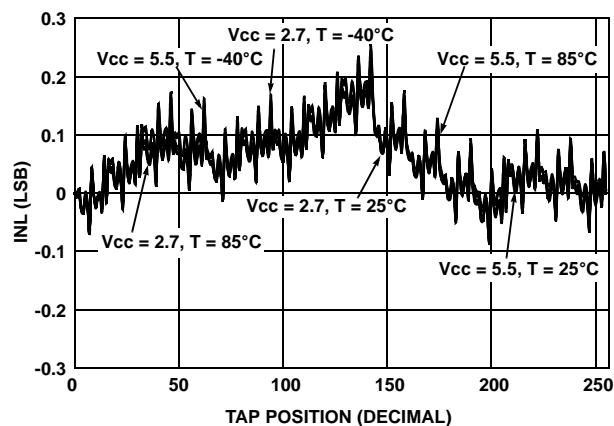
FIGURE 4. INL vs TAP POSITION FOR 10kΩ (W)
