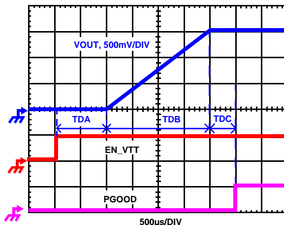
FIGURE 12. AMD SOFT-START WAVEFORMS
