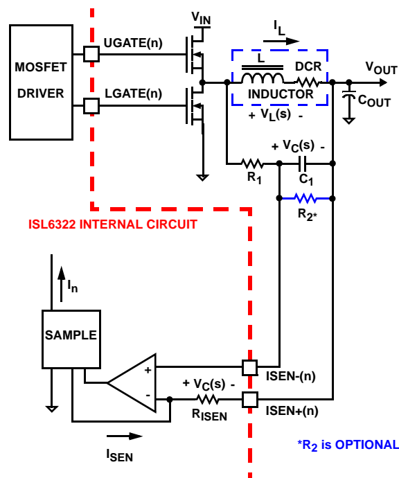
FIGURE 21. DCR SENSING CONFIGURATION
