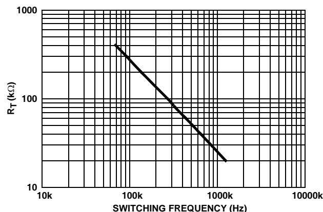
FIGURE 25. R_T vs SWITCHING FREQUENCY
