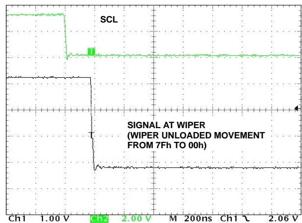
FIGURE 14. LARGE SIGNAL SETTLING TIME
