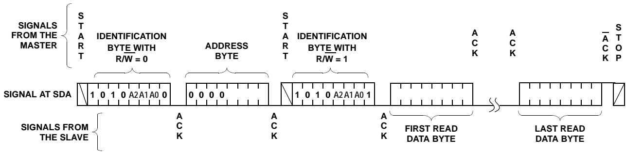
FIGURE 19. READ SEQUENCE
