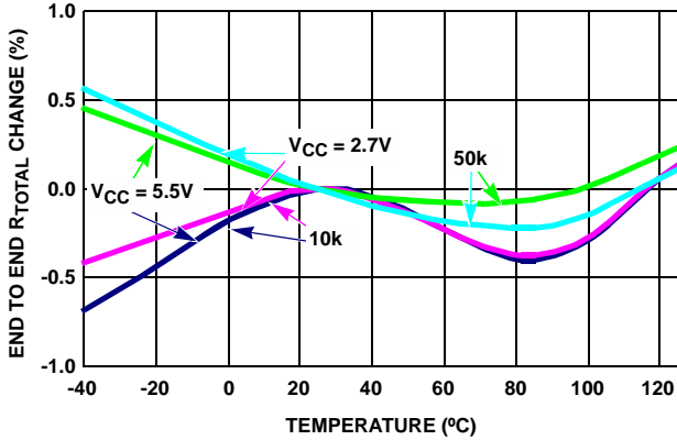
FIGURE 9. END TO END R_{TOTAL} % CHANGE vs TEMPERATURE
