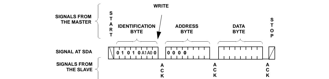
FIGURE 14. BYTE WRITE SEQUENCE
