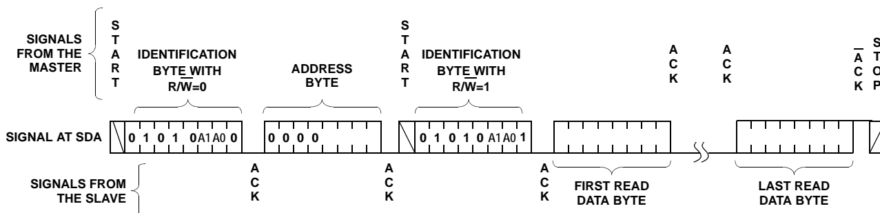
FIGURE 15. READ SEQUENCE
