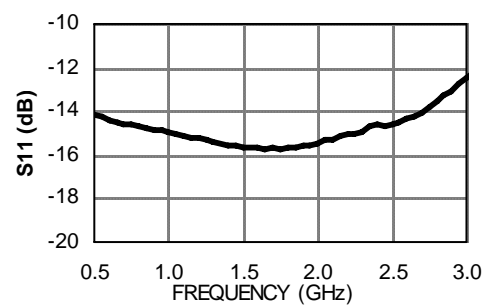
FIGURE 4. |S11| vs FREQUENCY
