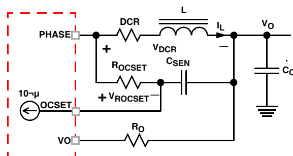
FIGURE 5. OVERCURRENT PROGRAMMING CIRCUIT
