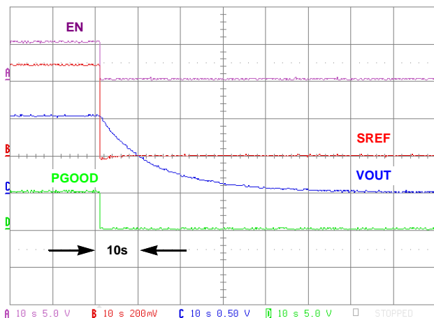
FIGURE 19. SHUT-DOWN, V_{IN} = 12.6V , V_{OUT} = 1.05V , LOAD = OPEN-CIRCUIT
