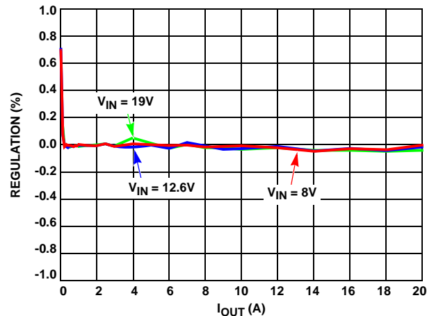
FIGURE 14. LOAD REGULATION AT V_{OUT} = 1.1V
