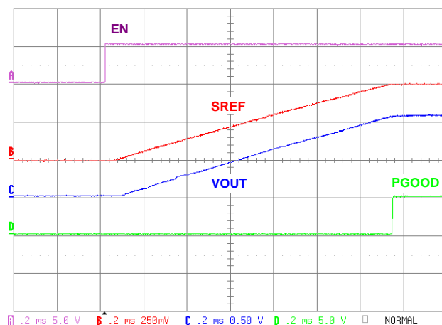
FIGURE 16. START-UP, V_{IN} = 12.6V , V_{OUT} = 1.05V , LOAD = 10A
