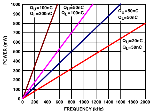
FIGURE 11. POWER DISSIPATION vs FREQUENCY
