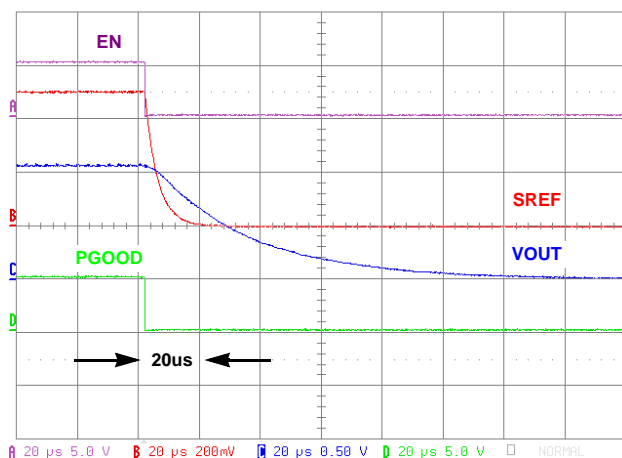
FIGURE 18. SHUT-DOWN, V_{IN} = 12.6V , V_{OUT} = 1.05V , LOAD = 50mΩ
