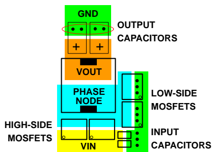
FIGURE 12. TYPICAL POWER COMPONENT PLACEMENT
