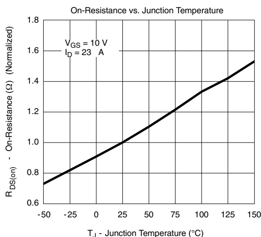
Fig. 7 MOSFET R_{DS(on)} vs. Temperature
