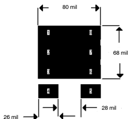
FIGURE 2. Footprint With Copper Spreading
