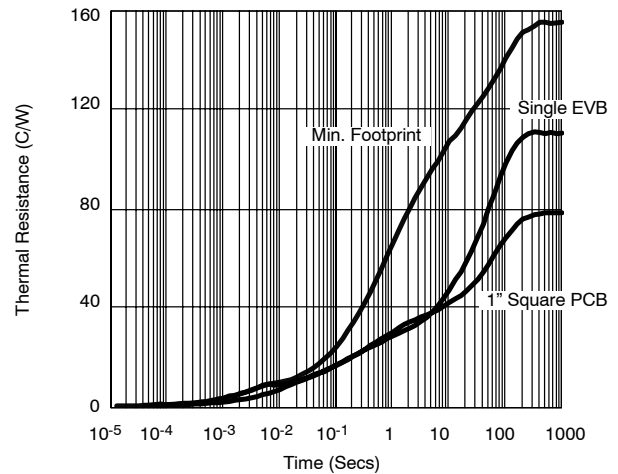
FIGURE 4. Single 1206-8 ChipFET
