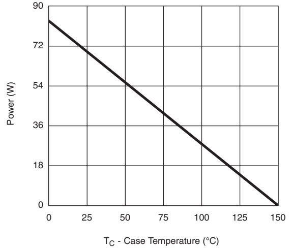
T_C - Case Temperature (°C) Power Derating, Junction-to-Foot
